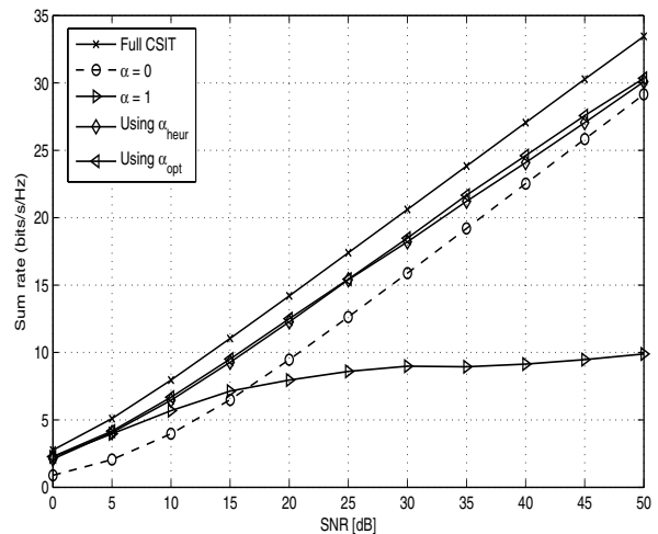
Figure 2: Sum capacities for M = 2 , K = 30 , B_{total} = 120 bits, and different schemes. \alpha_{heur} provides a smooth transition between extreme \alpha 's, with tolerable loss with respect to \alpha_{opt} .
