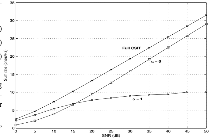
Figure 1: Sum capacities for M = 2, K = 20, B_{total} = 80 bits.
