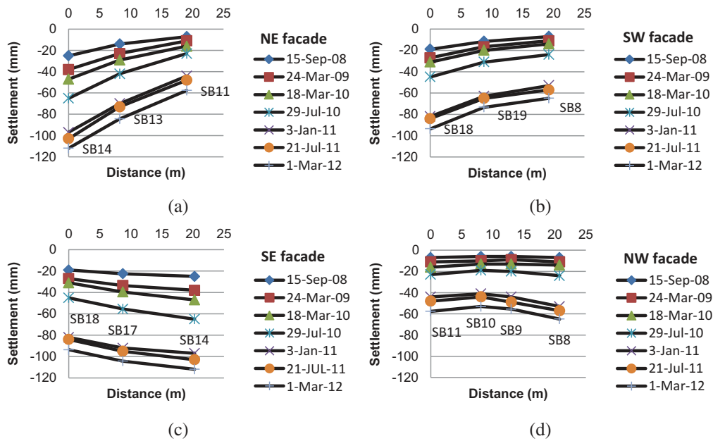
Figure 7. Monitored settlements along the main masonry walls.
