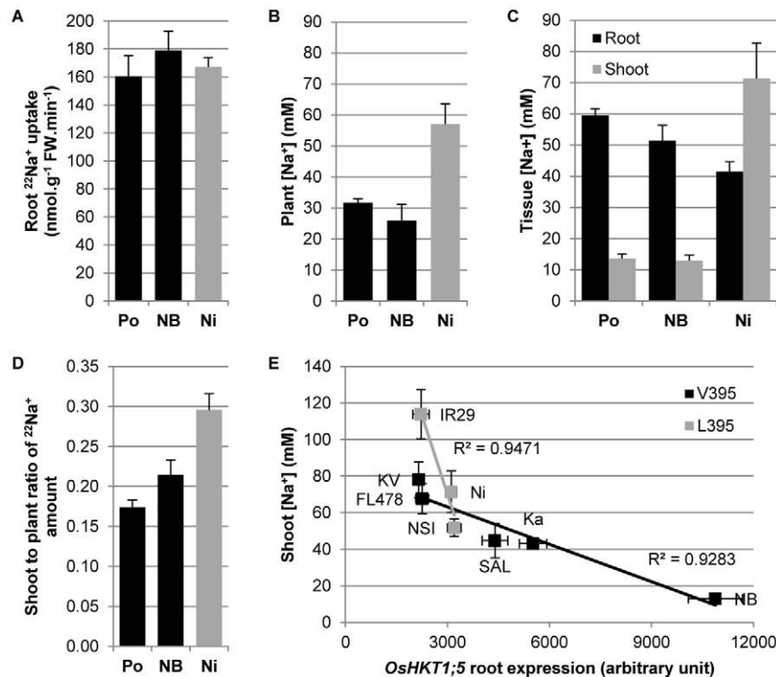
Figure 1. Root-to-shoot \text{Na}^+ transfer control in rice upon salt stress. (A) Radioactive ^{22}\text{Na}^+ fluxes measurement of root \text{Na}^+ uptake (+SEM; n=8 ) (uptake: 2 min). (B) Flame photometry measurement of plant total \text{Na}^+ concentration (+SEM; n=5 ). (C) Flame photometry measurement of tissue \text{Na}^+ concentrations (+SEM; n=5 ). (D) Radioactive ^{22}\text{Na}^+ fluxes measurement of the shoot-to-plant ratio of \text{Na}^+ amount (+SEM; n=8 ). (E) Correlation between root OsHKT1;5 expression level measured by qRT-PCR (three biological replicates per line \pm SEM; three technical replicates per biological sample) and shoot \text{Na}^+ concentration measured by flame photometry ( \pm SEM; n=5 ) in salt treated rice lines with either a Leu or a Val residue in position 395 of the OsHKT1;5 gene. The abbreviations Po= Pokkali; NB= Nona Bokra; Ni= Nipponbare; KV= Kallurundai Vellai; Ka= Kalurundai; NSI= NSICRC106; and SAL= SAL208 stand for individual varieties, variously represented through the panels A–E. IR29 and FL478 are full names of rice varieties.
