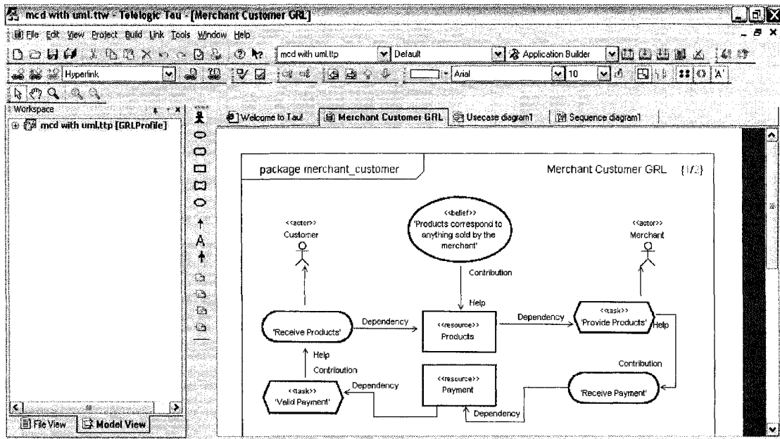
Figure 81 GRL Diagram in GRL Editor
