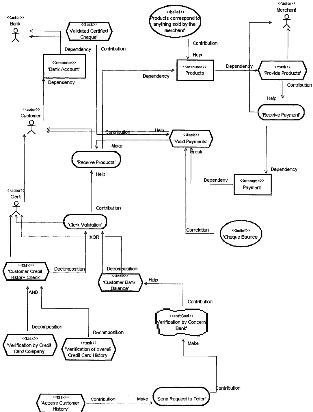
Figure 75 Merchant and Customer Dependencies, Modelled with Tau GRL Profile
