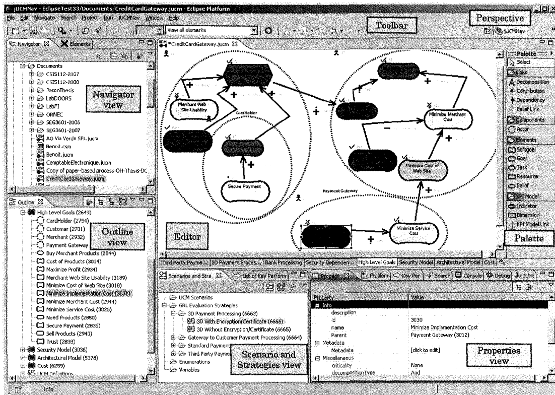
Figure 65 jUCMNav Editor View ([19])
