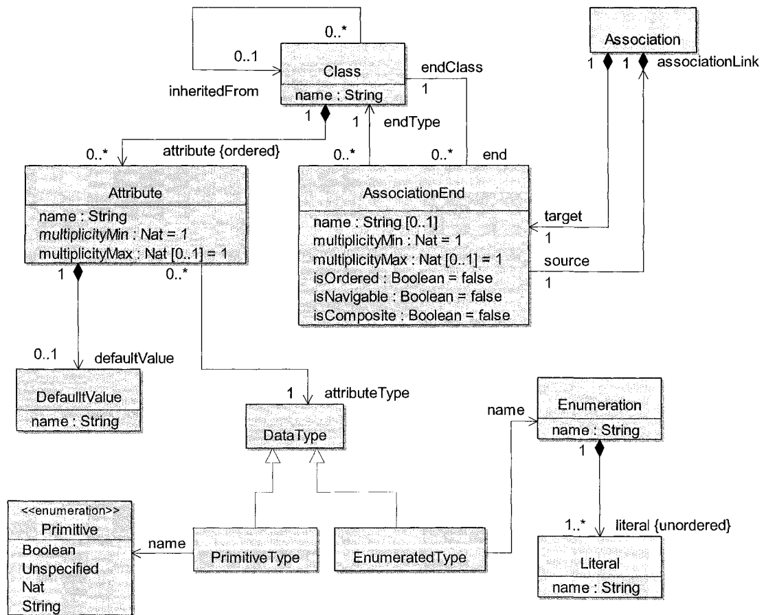
Figure 9 Z.111 Meta-metamodel
