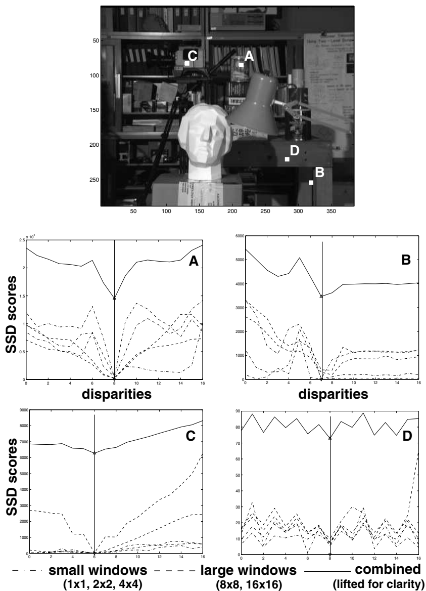
Fig. 4. Correlation curves for different points of the Tsukuba stereo pair. Case A represents a typical, well-textured, image point for which SSD would yield correct results for any window size. Case B shows a point close to a discontinuity where SSD with larger windows would fail. Case C and D show low-texture areas where small windows do not capture sufficient information for reliable consistency measures.
