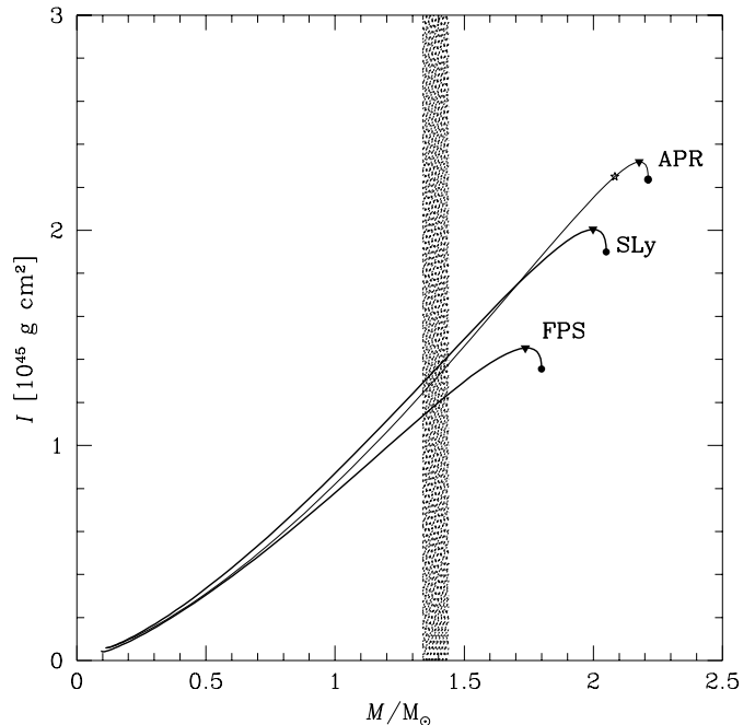
Fig. 9. Moment of inertia for slow, rigid rotation versus gravitational mass. The configuration with maximum I is indicated by a filled triangle, and that of maximum mass – by a filled circle. A shaded band corresponds to the range of precisely measured masses of binary radio pulsars.
