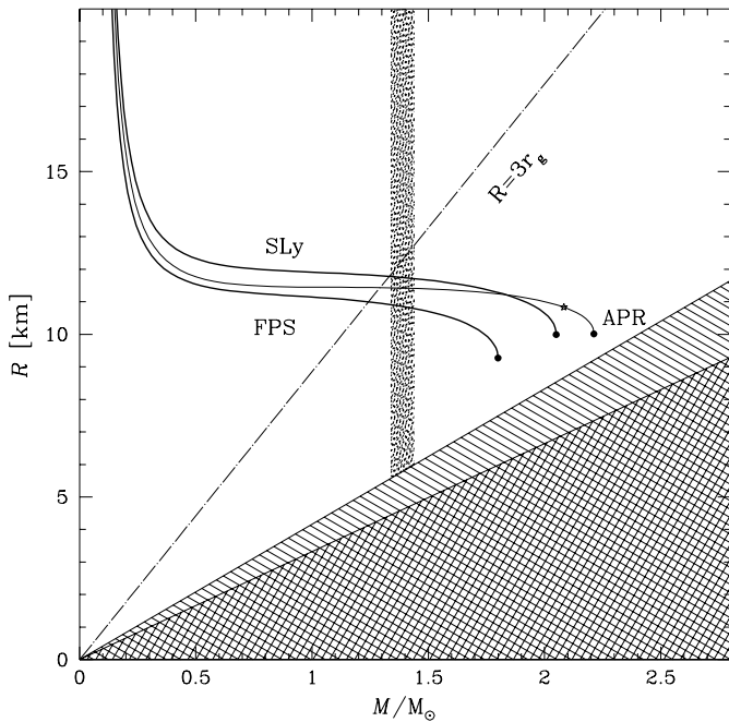
Fig. 6. Neutron star radius R versus gravitational mass M , with notation as in Fig. 4. Doubly hatched area is prohibited by general relativity, because it corresponds to R < \frac{9}{8}r_g = 9GM/4c^2 (for a general proof, see Weinberg 1972). All hatched triangle (double and single hatched) is prohibited by the general relativity and condition v_{\text{sound}} < c (necessary but not sufficient for respecting causality, Olsson 2000) combined. The shaded band corresponds to the range of precisely measured masses of binary radio pulsars.
