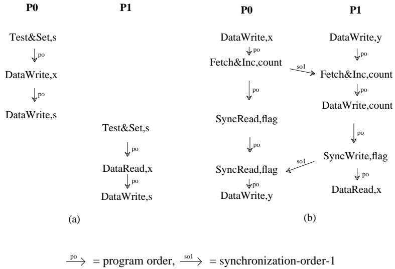
Figure 3. Executions that (a) exhibit and (b) do not exhibit data races.
