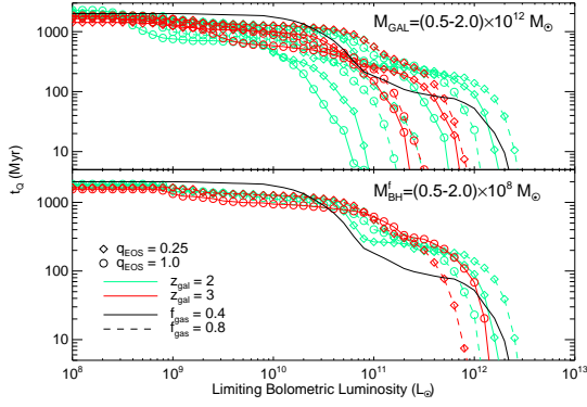
FIG. 4.— Integrated intrinsic quasar lifetime above a given reference bolometric luminosity, t_Q(L) , as a function of luminosity for simulations with host galaxies with total mass (top panel) M_{\text{gal}} = 0.5 - 2.0 \times 10^{12} M_{\odot} , and simulations with final black hole masses (bottom panel) M_{\text{BH}}^f = 0.5 - 2.0 \times 10^8 M_{\odot} (i.e. similar peak luminosity L_{\text{peak}} \sim 10^{12} L_{\odot} ). The simulations cover a range in equation of state parameter q_{\text{EOS}} , initial disk gas fraction f_{\text{gas}} , galaxy redshift (for scaling of halo properties) z_{\text{gal}} , and virial velocities V_{\text{vir}} = 113 - 160 \text{ km s}^{-1} . The black line in both cases is for a merger involving Milky Way-like galaxy models, which we refer to as A3, with f_{\text{gas}} = 1 , q_{\text{EOS}} = 1 , z_{\text{gal}} = 0 , and V_{\text{vir}} = 160 \text{ km s}^{-1} .
