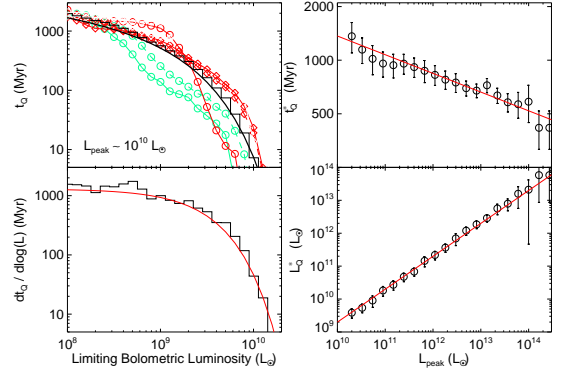
FIG. 5.— Fits to the quasar lifetime as a function of luminosity from our simulations. Upper left shows the intrinsic, bolometric quasar lifetime t_Q of a set of simulations with L_{\text{peak}} within a factor of 2 of 10^{10} L_{\odot} , in the manner of Figure 4. The black histogram shows the geometric mean of these lifetimes, and the black histogram in the lower left shows the differential lifetime dt/d\log L from this geometric mean. The black thick line in the upper left and red line in the lower left show the best-fit to our analytical form, dt/d\log L = t_Q^* \exp(-L/L_Q^*) . Upper right shows the fitted t_Q^* and resulting errors in each peak luminosity (final black hole mass) interval, and the best-fit power-law to t_Q^*(L_{\text{peak}}) (red line). Lower right shows the fitted L_Q^* and resulting errors in each peak luminosity (final black hole mass) interval, and the best-fit proportionality L_Q^* \propto L_{\text{peak}} (red line).
