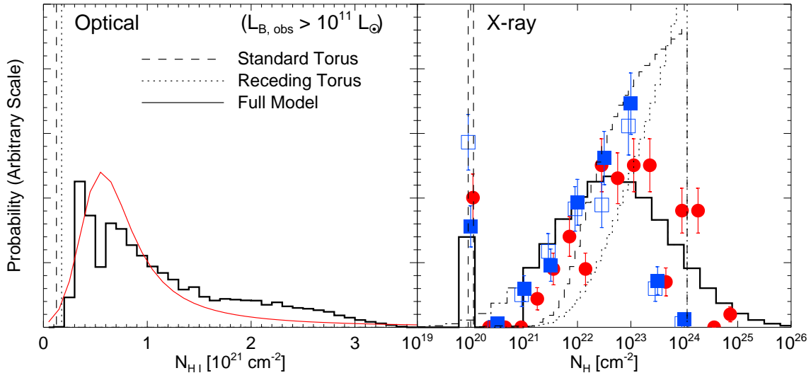
FIG. 12.— Left panel: Distribution of column densities expected from the characteristic quasars L_{\text{peak}} \sim L_* of the luminosity function observed in optical samples, for a standard torus model of quasar obscuration (dashed), a receding torus model (dotted), and the distributions of column densities as a function of instantaneous and peak luminosity in our simulations (solid). The distribution of neutral N_{\text{HI}} values is obtained requiring an observed B-band luminosity > 10^{11} L_{\odot} . The smooth red curve is the best-fit to the E_{B-V} distribution of bright SDSS quasars with z < 2.2 , from Hopkins et al. (2004), rescaled to column densities and plotted about a peak (mode) N_{\text{HI}} (undetermined in Hopkins et al. 2004) of N_{\text{HI}} \approx 0.5 \times 10^{21} \text{ cm}^{-2} . The i -band absolute magnitude limit imposed in the observed sample, M_i < -22 , corresponds approximately to our plotted B-band limit L_{B,\text{obs}} > 10^{11} L_{\odot} . Right panel: Integrated distribution of total (neutral and ionized) column densities expected for a complete hard X-ray sample, from the column densities of our simulations and the n(L_{\text{peak}}) distribution. The distribution below 10^{21} \text{ cm}^{-2} is shown (dot-dashed line) and re-plotted as a single bin at N_{\text{HI}} = 10^{20} \text{ cm}^{-2} for our modeled columns. Data shown are the results of Treister et al. (2004) (blue squares) and Mainieri et al. (2005) (red circles), with assumed Poisson errors. Solid squares assume an intrinsic photon index \Gamma = 1.9 , for the soft X-ray quasar spectrum, open squares \Gamma = 1.7 .
