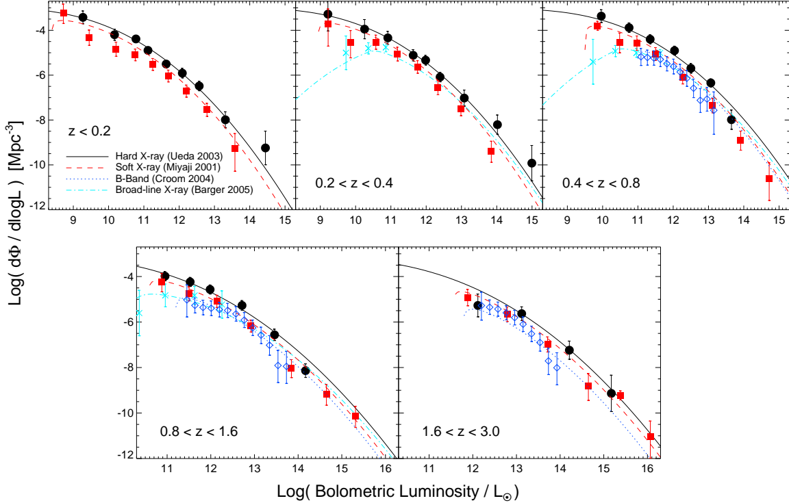
FIG. 9.— Best-fit luminosity function from the pure peak-luminosity evolution n(L_{\text{peak}}) distribution, for redshifts z = 0-3 . From our fitted lognormal n(L_{\text{peak}}) distribution, we simultaneously reproduce the luminosity function in the hard X-ray (2-10 keV; solid black line), soft X-ray (0.5-2 keV; dashed red line), and optical B-band (4400 Å; dotted blue line) at all redshifts. Moreover, we reproduce the distribution of broad-line quasars in hard X-ray selected samples (cyan dot-dashed line), as described in § 4. All quantities have been rescaled to bolometric luminosities for ease of comparison, using the corrections of Marconi et al. (2004), with the plotted error bars representing both quoted measurement errors and the estimated errors in the bolometric corrections. The observations are from Miyaji et al. (2001) (soft X-ray; red squares), Ueda et al. (2003) (hard X-ray; black circles), Croom et al. (2004) (B-band, blue diamonds), and Barger et al. (2005) (X-ray selected broad-line quasars; cyan crosses).
