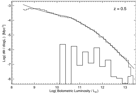
FIG. 8.— We reproduce (thin histogram) the luminosity function of Ueda et al. (2003) at redshift z = 0.5 (thin curve) using the binned differential quasar lifetime dt/d\log L directly from our simulations and a fitted distribution of peak luminosities \dot{n}(L_{\text{peak}}) (thick histogram). For each bin in \log(L_{\text{peak}}) , we average the binned differential lifetime of a set of simulations with peak luminosity in the bin. This clearly demonstrates our key qualitative result, that the faint end of the luminosity function is reproduced by quasars with peak luminosity around the break luminosity but observed primarily in sub-Eddington states (luminosities L \ll L_{\text{peak}} ), is not an artifact of our fitting formulae or extrapolation to extreme luminosities.
