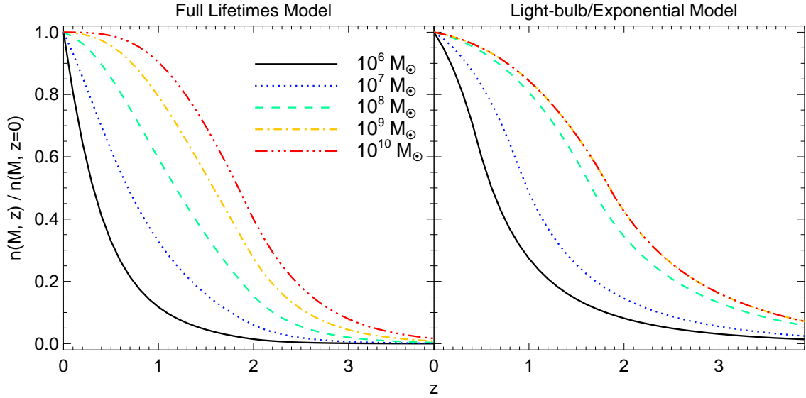
FIG. 23.— Fractional number density n(M, z)/n(M, z=0) of black holes of a given mass as a function of redshift, for several different black hole masses as shown. For z > 2 this includes the turnover (pure density evolution form) in the quasar space density above z = 2 from high-redshift luminosity functions described in § 3.2. Left panel shows the results using our full model of quasar lifetimes, right panel assuming a “light-bulb” or exponential (constant Eddington ratio) light curve model. The yellow dot-dash ( 10^9 M_{\odot} ) and red triple-dot-dash ( 10^{10} M_{\odot} ) curves are nearly identical in the right panel.
