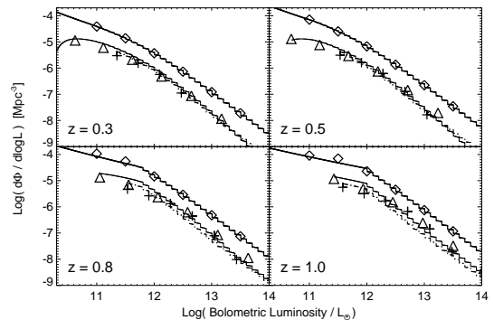
FIG. 10.— Hard X-ray (thick), soft X-ray (thin), and B-band (dot-dash) LFs determined from our model of quasar lifetimes and column densities, based on a distribution of intrinsic source properties fitted to the observed hard X-ray LF and the limiting magnitudes of observed samples, at the different redshifts shown. All quantities are rescaled to bolometric luminosities with the bolometric corrections of Marconi et al. (2004). Symbols show the observed LFs for hard X-rays (Ueda et al. 2003, diamonds), soft X-rays (Miyaji et al. 2000, triangles), and B-band (Boyle et al. 2000, crosses). Reproduced from Hopkins et al. (2005d).
