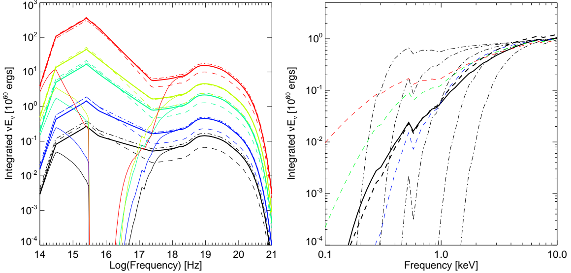
FIG. 24.— Left: Integrated intrinsic spectra (thick solid lines) from simulations A1, A2, A3, A4, and A5 (black, blue, green, yellow, red, respectively), with virial velocities V_{\text{vir}} = 80, 113, 160, 226, and 320 \text{ km s}^{-1} . The predicted integrated spectra from our model for quasar lifetimes are shown as dot-dashed lines, and the prediction of a “light bulb” model, where the same total energy is radiated at L = L_{\text{peak}} , as dashed lines. Integrated observed spectra are shown as thin solid lines. Right: Integrated observed X-ray spectrum from the A3 simulation (thick black line), compared with the integrated intrinsic spectrum, reddened by various column density distributions: our fitted N_{\text{H}} distributions from § 2.3 (thick black dashed line), constant (luminosity-independent) lognormal N_{\text{H}} distribution with \bar{N}_{\text{H}} = 10^{22} \text{ cm}^{-2} and \sigma_{N_{\text{H}}} = 0.4, 0.7, 1.0 (blue, green, and red dashed lines, respectively), and constant N_{\text{H}} = 10^{21}, 10^{21.5}, 10^{22}, 10^{22.5}, and 10^{23} \text{ cm}^{-2} (thin dot-dashed lines).
