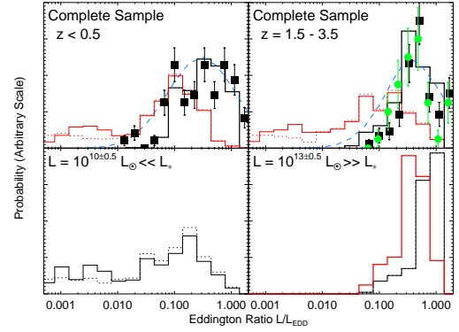
FIG. 20.— Predicted distribution of Eddington ratios based on the luminosity function and the quasar evolution in our simulations, in two redshift intervals z < 0.5 (upper left) and 1.5 < z < 3.5 (upper right). The observed distributions for radio loud (black squares) and radio quiet (green circles) quasars are shown from Vestergaard (2004) with Poisson errors. Thick black lines show the predicted distribution given the same minimum observed luminosity as the observed sample. Thin red lines show the predicted distributions for a sample extending to arbitrarily faint luminosities, dotted lines show the same, with the ADAF correction of § 5 applied at low accretion rates. Blue dashed lines show the prediction for a fixed (luminosity-independent) Eddington ratio distribution in a light-bulb or exponential light curve model, fitted to the z < 0.5 data and used to predict the 1.5 < z < 3.5 Eddington ratio distribution given the observational luminosity limit. Lower panels show the predicted distributions for z \lesssim 1 in two luminosity intervals, above and below the “break” luminosity in the observed luminosity function (red lines here correspond to an observed (attenuated) B-band luminosity L_{B,\text{obs}} > 10^{11} L_{\odot} ).
