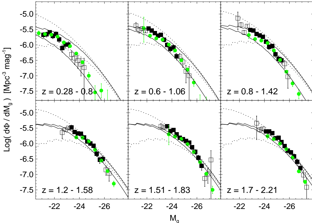
FIG. 15.— Broad-line quasar luminosity function of Richards et al. (2005) from the 2dF-SDSS (2SLAQ) survey (black squares) and that of Croom et al. (2004) (green circles) from the 2dF survey, compared to our predicted “broad-line” luminosity function from our determination of the relative quasar and host galaxy luminosities in our simulations (solid line), where we estimate that quasars are observable as “broad-line” objects when their observed B-band luminosity is greater than a factor f_{\text{BL}} of that of the host galaxy. Solid lines are shown for the minimum and maximum observed redshift in each bin (as labeled), assuming f_{\text{BL}} = 1 . Dotted lines show the result for f_{\text{BL}} = 0.3 and f_{\text{BL}} = 3 , at the mean redshift of the bin, i.e. corresponding to “broad-line” luminosity functions in surveys which are complete to quasars with observed optical luminosity \sim 0.3 and 3 times that of the host galaxy, respectively, or alternatively reflecting nearly complete theoretical uncertainty regarding merging galaxy gas fractions ( f_{\text{gas}} = 0.1 - 0.9 ). Open squares are observations with uncertain incompleteness corrections in Richards et al. (2005).
