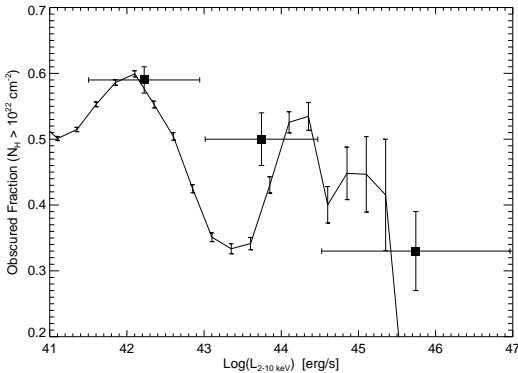
FIG. 17.— Predicted “obscured” fraction (solid line) in an X-ray sample with identical redshift and luminosity range to that of Ueda et al. (2003), as a function of hard X-ray (2–10 keV) luminosity. Vertical error bars show Poisson errors estimated from the total time at a given luminosity across all our simulations (absolute values of the error bars should not be taken literally). The “obscured” fraction is defined as the fraction of quasars with X-ray column densities N_{\text{H}} > 10^{22} \text{ cm}^{-2} in bins of \Delta \log L_{2-10 \text{ keV}} . The observations from Ueda et al. (2003) are shown as black squares.
