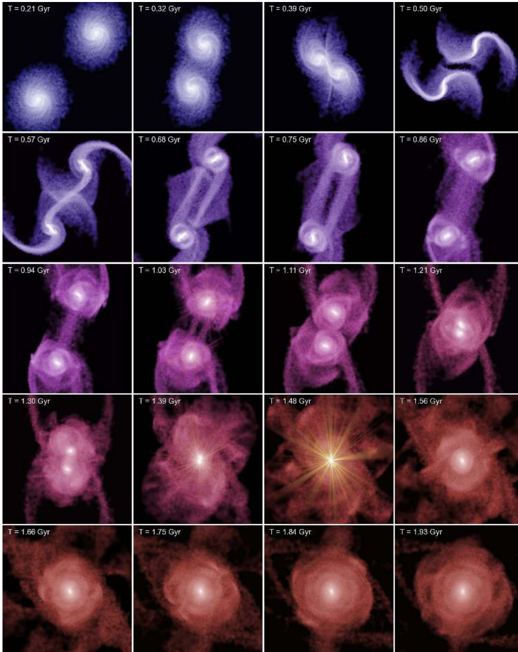
FIG. 2.— Time sequence from one of our merger simulations ( V_{\text{vir}} = 160 \text{ km s}^{-1} , initial gas fraction 20%). Each panel is 80 h^{-1} \text{ kpc} on a side and shows the simulation time in the upper left corner. Brightness of individual pixels gives the logarithm of the projected stellar mass density, while color hue indicates the baryonic gas fraction, from 20% (blue) to less than 5% (red). At T = 1.03, 1.39 and 1.48 \text{ Gyr} , when the black hole could be seen as an optical quasar, nuclear point sources are shown, providing a representation of the relative luminosities of stars and the quasar at these times.
