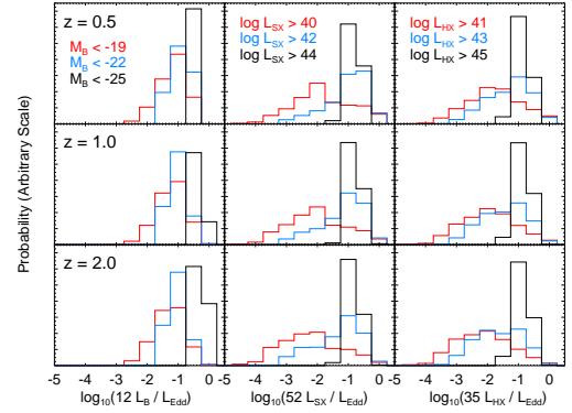
FIG. 21.— Predicted distribution of Eddington ratios based on the luminosity function and the quasar evolution in our simulations, at three redshifts z = 0.5 (top panels), z = 1.0 (middle), and z = 2.0 (bottom). The inferred distribution of Eddington ratios, adopting a constant bolometric correction from the observed (attenuated) luminosity in each of three bands is shown, i.e. assuming L = 12 L_B^{obs} (4400 Å; left), L = 52 L_{SX}^{obs} (0.5–2 keV; middle), and L = 35 L_{HX}^{obs} (2–10 keV; right). For each waveband, results are shown for three reference luminosities. In B-band, M_B < -19 (red), M_B < -22 (blue), and M_B < -25 (black). In soft X-rays, \log(L_{SX}[\text{erg s}^{-1}]) > 40 (red), 42 (blue), 44 (black). In hard X-rays, \log(L_{HX}[\text{erg s}^{-1}]) > 41 (red), 43 (blue), 45 (black).
