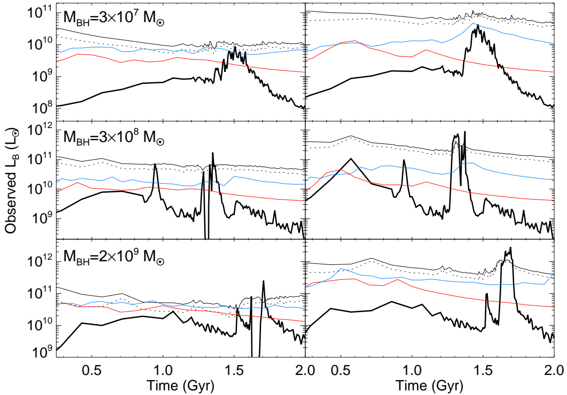
FIG. 13.— Intrinsic (right panels) and median attenuated (left panels) B-band luminosity of the quasar (thick line) and host galaxy (integrated over all stars, thin line; ignoring bulge stars, dotted line) as a function of time. Results are shown from three representative simulations: A2, A3, and A5 (see § 2.1) with q_{\text{EOS}} = 1.0 , z_{\text{gal}} = 0 , and virial velocities V_{\text{vir}} = 113, 160 , and 320 \text{ km s}^{-1} . Each quasar should be observable as a broad-line AGN when L_{\text{B, QSO}} \gtrsim L_{\text{B, host}} . Colors show the stellar light curve with different gas fractions f_{\text{gas}} = 1.0 (black), f_{\text{gas}} = 0.4 (blue), and f_{\text{gas}} = 0.2 (red); quasar light curves are similar for each gas fraction.
