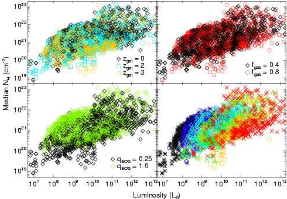
FIG. 3.— The median fitted total (neutral and ionized) column density \bar{N}_H at each luminosity L in the snapshots from our series of simulations described in § 2. We compare changing concentrations and halo properties with redshift z_{\text{gal}} (upper left), gas fractions f_{\text{gas}} (upper right), the equation of state parameter q_{\text{EOS}} (lower left), and virial velocity V_{\text{vir}} (lower right). At lower right, simulations with V_{\text{vir}} = 80, 113, 160, 226, 320, and 500 \text{ km s}^{-1} are shown as black asterisks, purple dots, red diamonds, green triangles, yellow squares, and red crosses, respectively. Other than a possible weak sensitivity to q_{\text{EOS}} , the column density distribution as a function of luminosity shows no systematic dependence on any of the varied simulation parameters.
