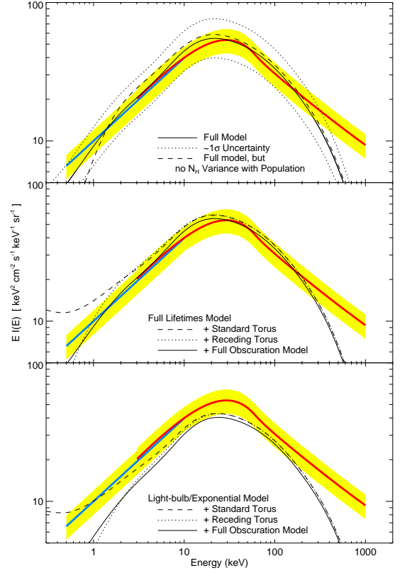
FIG. 25.— Predicted integrated X-ray background spectrum (solid black line) from our model of quasar lifetimes and attenuation, with the peak luminosity distribution \dot{n}(L_{\text{peak}}) determined from the luminosity function. Blue and red thick lines show the observed spectrum from Barcons et al. (2000) and Gruber et al. (1999), respectively. The shaded yellow area illustrates the uncertainty in normalization between both samples (alternatively, 2\sigma errors in the Barcons et al. 2000 normalization). The predictions given 1\sigma deviations in the fitted \dot{n}(L_{\text{peak}}) distribution (dotted lines) and given the \dot{n}(L_{\text{peak}}) distribution determined from hard X-ray data only (dashed line) are shown in the upper panel. Middle panel shows the prediction using our modeling of quasar lifetimes but different models of obscuration, lower panel the prediction with a “light-bulb” or exponential (constant Eddington ratio) model and different obscuration models.
