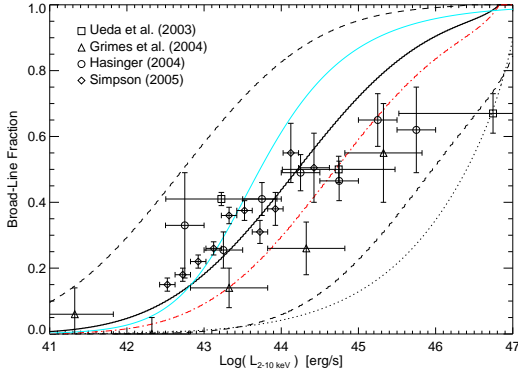
FIG. 16.— Predicted “broad-line” fraction of a complete X-ray sample at low z \lesssim 0.3 redshift, from our simulations (where the object is observable as a broad-line quasar when it has an observed B-band luminosity greater than a factor f_{\text{BL}} = 1.0 of that of its host galaxy), is shown (thick black line). The results, changing our f_{\text{BL}} to 0.3 and 3.0 are shown, or equivalently of assuming a host galaxy gas fraction f_{\text{gas}} = 0.1 or 0.9 instead of \sim 0.3 (dashed), as are the results assuming a “light bulb” model where quasars spend a fixed time t_Q = 20 Myr as broad line objects with a luminosity of L_{\text{peak}} (dotted). For comparison, the (scaled to 2–10 keV luminosity) observations of Ueda et al. (2003) (squares), Hasinger (2004) (circles), Grimes, Rawlings, & Willott (2004) (triangles), and Simpson (2005) (diamonds) are shown. The predicted result at higher redshift ( z \gtrsim 1 ) is shown (red dot-dashed line), offset owing to the shift in break luminosity of the luminosity function with redshift. The best-fit luminosity-dependent torus model, fitted to the data, is shown as the solid cyan line. The best-fit static torus model is a constant broad-line fraction \sim 0.3 (not shown for clarity).
