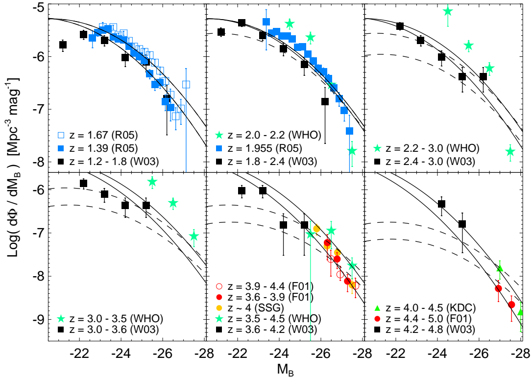
FIG. 11.— Running our predicted broad-line luminosity function (determined in § 3, 4) to high redshifts, with either total density (dashed lines) or break luminosity ( L_* ; solid lines) decreasing exponentially with redshift above z = 2 . In each panel, our prediction is shown for the minimum and maximum redshift of the corresponding interval from the COMBO-17 luminosity function of Wolf et al. (2003) (W03; black squares). Other references for the observations shown are: R05 - Richards et al. (2005), WHO - Warren et al. (1994), F01 - Fan et al. (2001), SSG - Schmidt, Schneider, & Gunn (1995), KDC - Kennefick, Djorgovski, & De Carvalho (1995).
