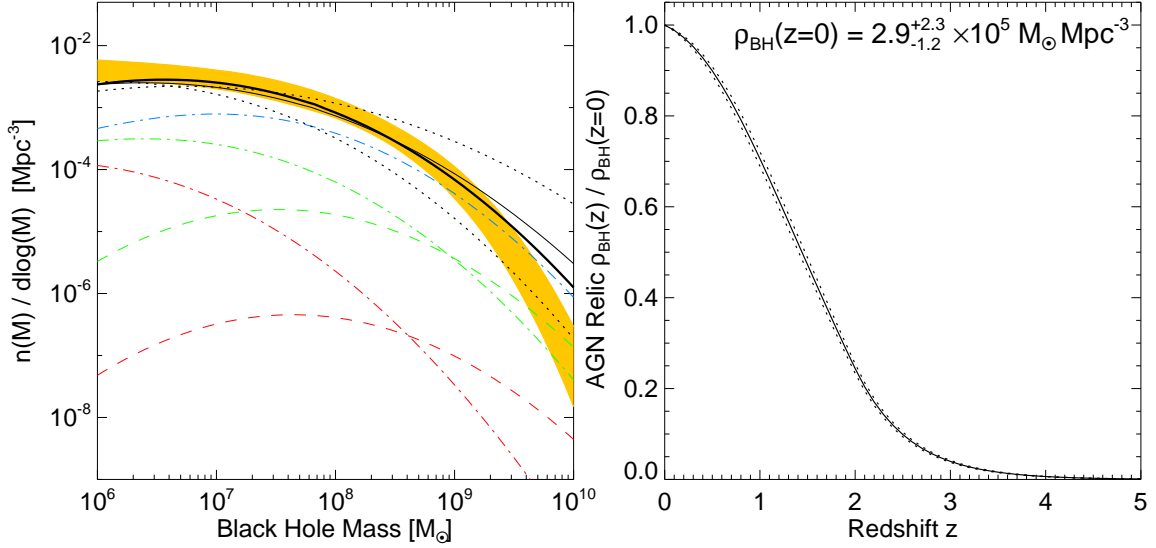
FIG. 22.— Right: Total predicted quasar relic black hole mass density and evolution of the fractional black hole mass density with redshift. Dotted lines show the difference resulting from 1\sigma deviation in fitted \dot{n}(L_{\text{peak}}) from the luminosity function. Left: Predicted present z=0 relic mass function (thick black line), for comparison with the 1\sigma range (yellow) of the inferred supermassive black hole mass function from Marconi et al. (2004). Also shown are the results given 1\sigma errors in the fitted \dot{n}(L_{\text{peak}}) distribution (dotted lines), or ignoring the small corrections to M_{\text{BH}}^f(L_{\text{peak}}) from § 2.4 (thin black line). Dot-dashed lines show the predicted mass function at z = 1.5, 3.0, 5.0 (blue, green, and red, respectively). The extensions to z > 2 includes the turnover (pure peak luminosity evolution form) in the quasar space density above z = 2 from high-redshift luminosity functions described in § 3.2, except for the dashed green and red lines which use the pure density evolution form.
