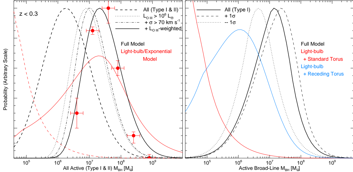
FIG. 18.— Predicted distribution of currently active black hole masses, both considering all types (Type I & II; left) and only those visible as broad-line quasars (Type I; right), at low z \lesssim 0.3 redshift, from our n(L_{\text{peak}}) distribution and the estimation of the “broad-line” phase directly from the simulations. In the left panel (all quasar types), we consider the result with arbitrarily faint luminosity limits (dashed line), and with the luminosity completeness limit (dotted) and both luminosity limit and velocity dispersion limit (dash-dot) of the SDSS sample of Heckman et al. (2004). We then consider the mass distribution with these limits, weighted by OIII luminosity, for direct comparison to the mass function of Heckman et al. (2004), shown as red circles (vertical errors represent the range in different parameterizations of the luminosity-weighted mass function from Heckman et al. (2004), their Fig. 1, horizontal errors a \sim 0.2 dex uncertainty in the black hole mass). Black lines show this for our full model, red lines show the full distribution (dashed) and distribution with the same weighting and selection effects as Heckman et al. (2004) (solid) for a light-bulb or exponential light curve model of quasar evolution. At right, the distribution of active “broad-line” quasar masses (solid, where an object is a “broad-line” quasar if the observed quasar B-band luminosity is above a factor f_{\text{BL}} = 1 of that of the host galaxy – dotted and dashed lines show the result if f_{\text{BL}} = 0.3 or 3, respectively). Black lines show the prediction of the full model, red and blue lines the predictions of a light-bulb/exponential light curve model with a standard torus model (red) and receding torus model (blue) used to determine the broad-line fraction.
