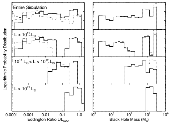
FIG. 19.— Distribution of Eddington ratios (left panels) and instantaneous black hole mass (right panels) as a function of quasar bolometric luminosity for our fiducial Milky Way-like A3 simulation, with V_{\text{vir}} = 160 \text{ km s}^{-1} and L_{\text{peak}} \sim 5 \times 10^{13} L_{\odot} . The trend of an increasingly narrow Eddington ratio and mass distribution (concentrated at higher values) with increasing luminosity is clear. The result of applying an ADAF-type radiative efficiency correction at low accretion rates is shown (dashed) as well as the result of considering only times after the final merger, with M_{\text{BH}} \sim M_{\text{BH}}^f (dotted).
