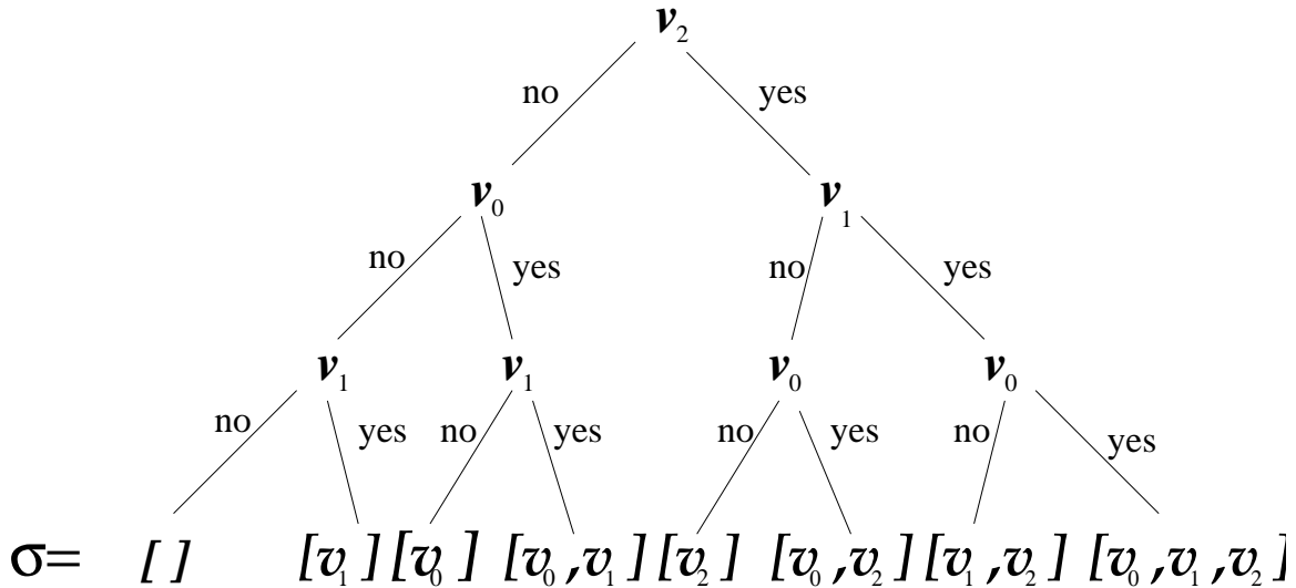
A guessing algorithm
