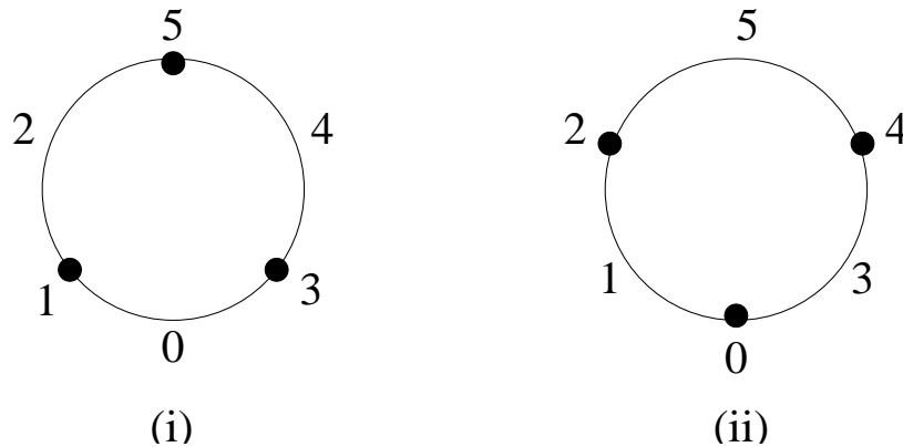
(i). This is not a discrete Morse function. (ii). This is a discrete Morse function.
