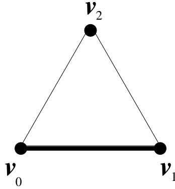
An example of an evasive subcomplex of the 2-dimensional simplex.
