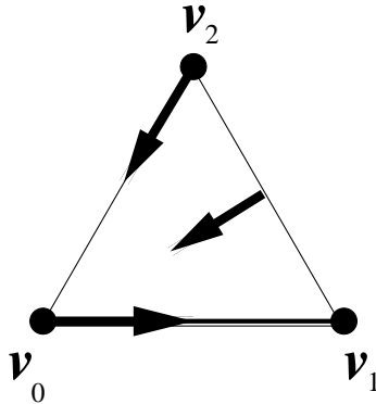
The vector field induced by the guessing algorithm shown in Figure 10.3.
