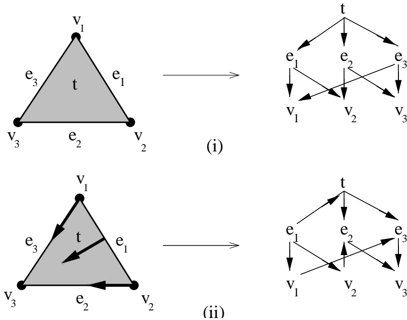
From a discrete vector field to a directed Hasse diagram.
