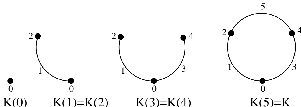
The level subcomplexes of the discrete Morse function shown in Figure 2.2(ii)
