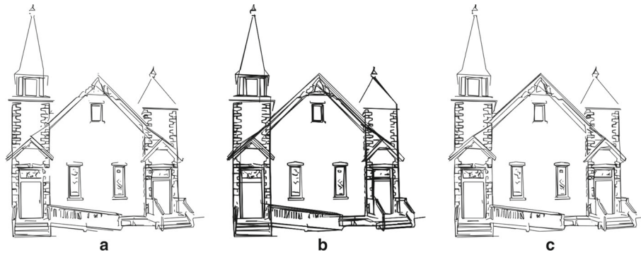
Fig. 8 Results of segment detection of the image in Fig. 7a. a Detected segments without considering segment endpoints of neighboring lines. b Detected segments without non-maximum suppression. c Detected segments using endpoints of neighboring lines and non-maximum suppression
