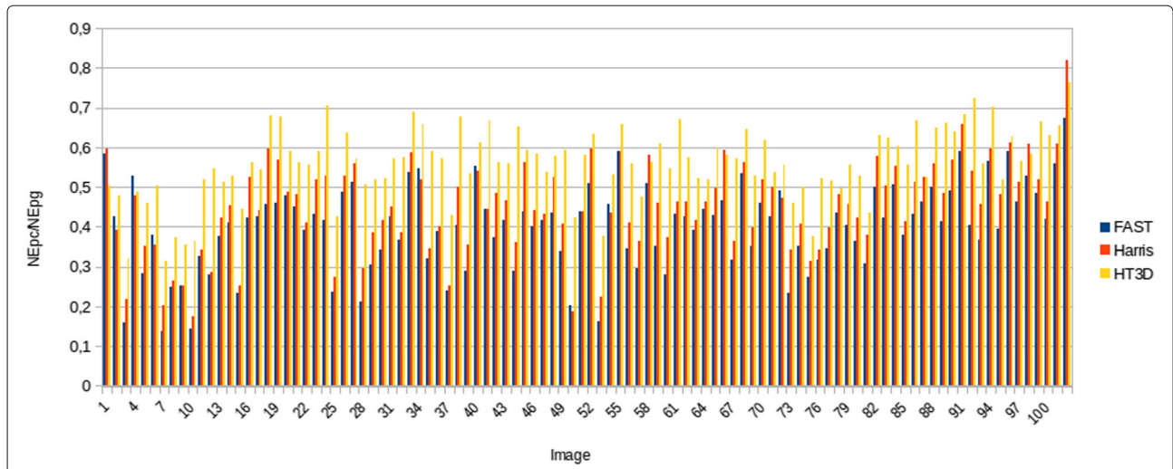
Fig. 18 Ratio between NEp_c (number of correct matchings between ground truth and detected points) and NEp_g (number of ground truth points) for the whole dataset considering d_{Ep} = 3 (distance between ground truth and detected points). This ratio quantifies the hit rates of the three corner detection methods. In general, clearly higher hit rates can be observed when using the proposed method in the large majority of the test images
