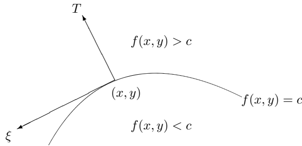
FIG. 2.1. A contour \mathcal{C} separating two homogeneous regions.
