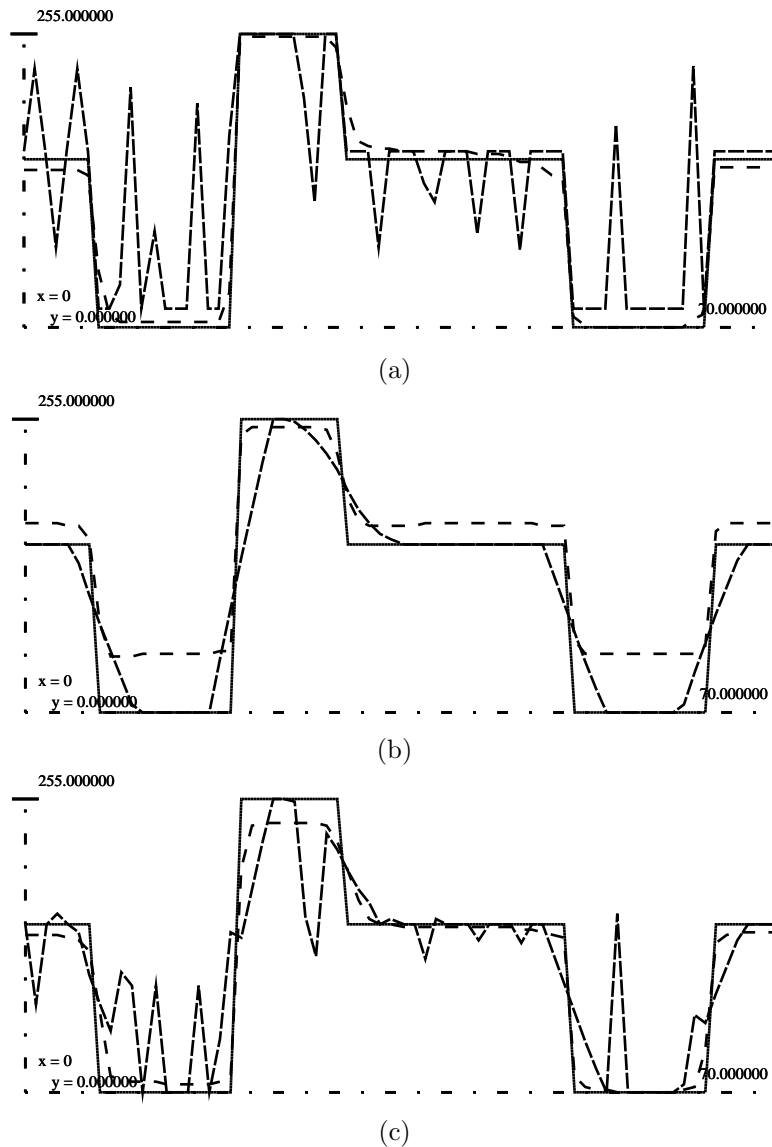
FIG. 7.2. Profiles of the synthetic image (—), the noisy initial image (---), and the reconstructed image (- · -), with the function \phi_1 . We represent in (a) the denoising case and in (b) the deblurring case; (c) involves both noise and blur.
