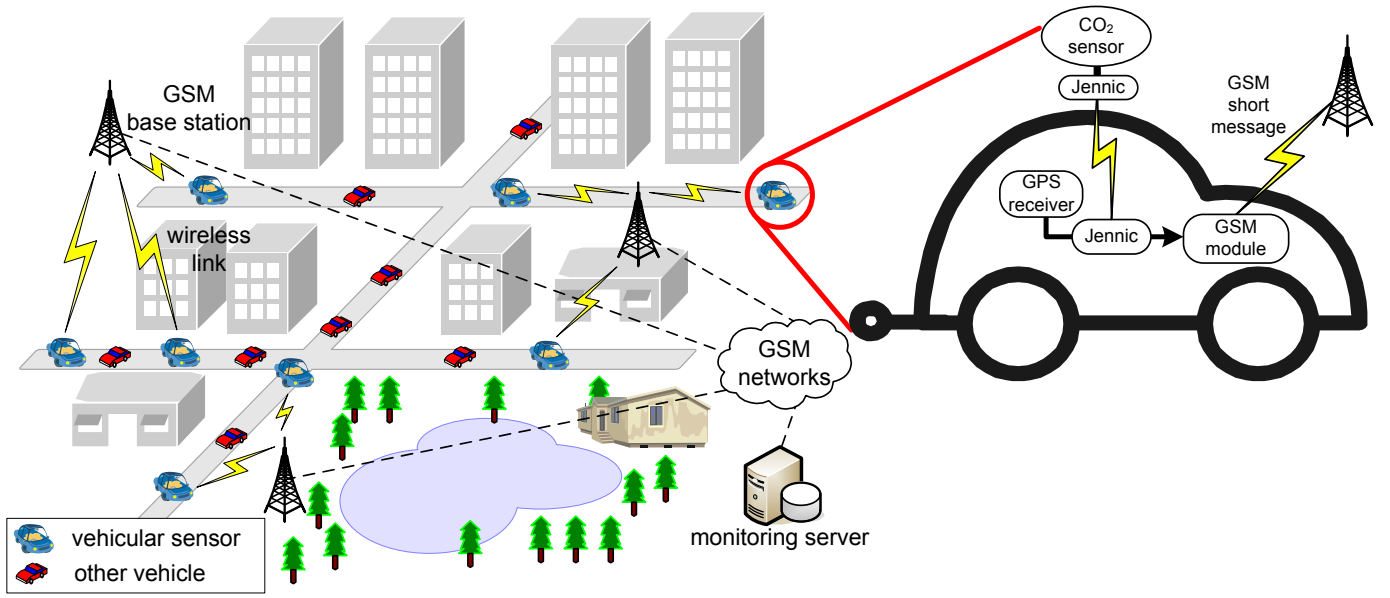
Fig. 1. The proposed VSN architecture for micro-climate monitoring.
