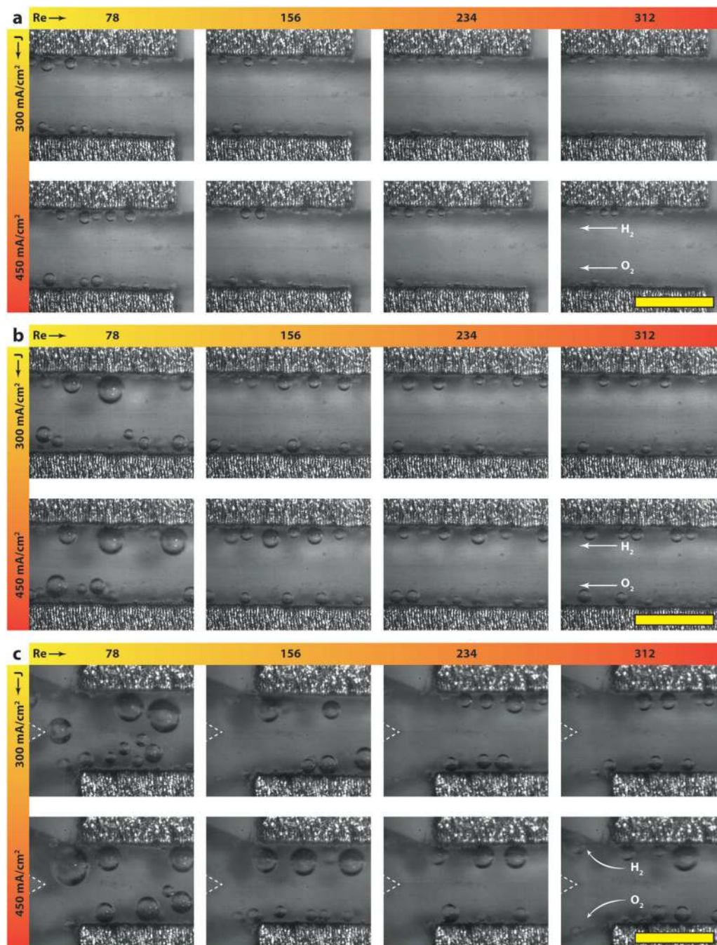
Fig. 3 Snapshots of the upstream (a), midstream (b), and downstream (c) regions of the electrolyzer: in general, the volume fraction and average size of bubbles increase with decreasing flow rate or increasing the current density. At low flow rates, some bubbles depart from the walls and move towards the center since the inertial forces are not strong enough. This phenomenon increases the crossover rate at these conditions as quantified by the GC results. The separating wedge is highlighted with a dashed triangle for better clarity in the downstream figures. The yellow scale bars at the corners are 1 mm in size.
