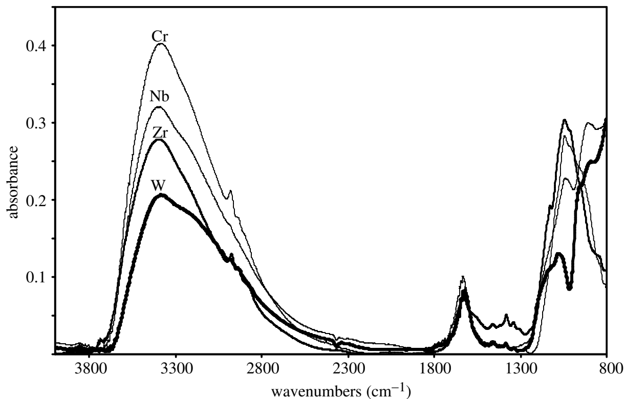
Figure 4. FTIR spectra of various M/Si=2 composites. The labels indicate the metal oxide present in each spectrum. The \nu_{as}(Si-O-Si) peak for the compounds can be seen c.a. 1050\text{ cm}^{-1} . Peaks at energies >1000\text{ cm}^{-1} for the Nb and W composites are due to the metal oxide phase as confirmed by FTIR analysis of samples containing no SiO_2 component.
