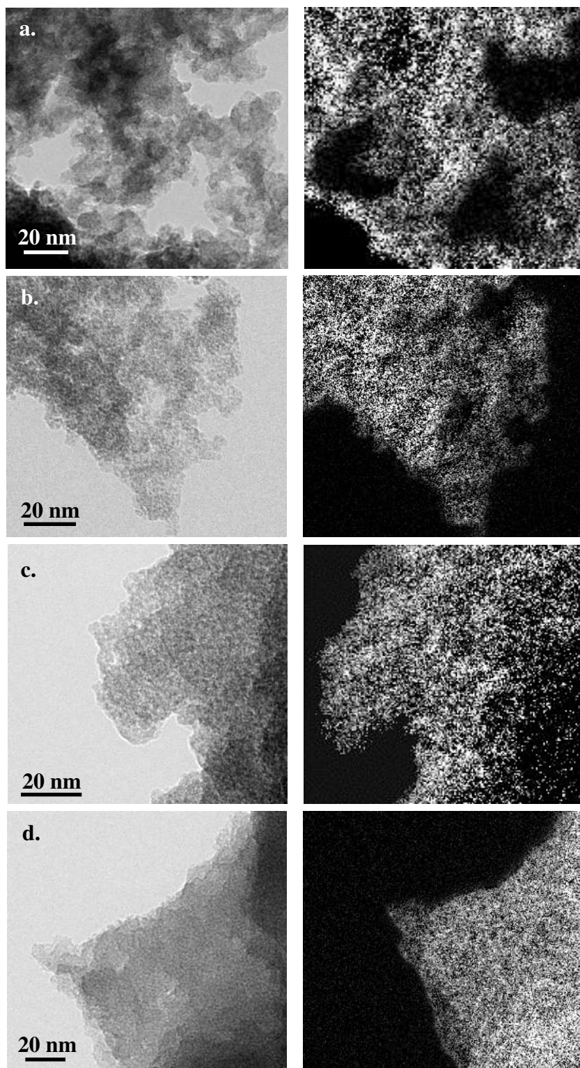
Figure 5. Bright field TEM images (left) and EFTEM Si maps (right) of a. W/Si = 2, b. Nb/Si=1, c. Zr/Si=1, and d. Cr/Si=2 aerogels.
