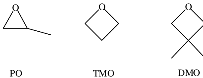
Figure 2. Structures of a 1,2-epoxide (PO) and 1,3-epoxides (TMO and DMO).
