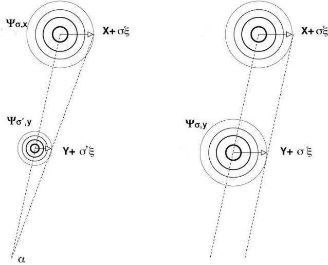
Figure 1. The function h that attains the supremum, in case \sigma > \sigma' and \sigma = \sigma' . Dot lines are tangent to the gradient of h .
