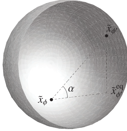
Figure 2. The vertical plane containing \bar{\mathbf{x}}_\phi, \bar{\mathbf{x}}_{\phi'} .
