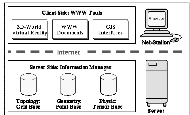
Figure 9 | Concept of WWW-based collaboration platform (TaiGer project).
