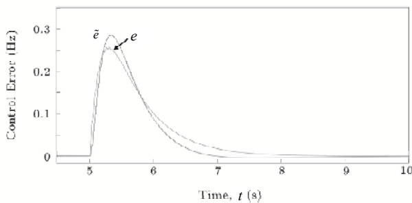
Figure 8. Estimated control error for random variation in parameters.
