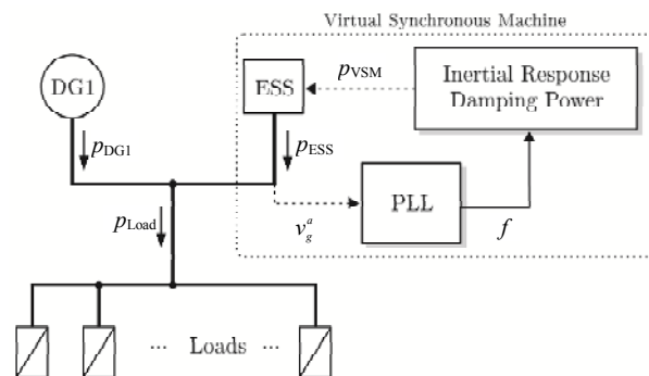
Figure 2. Diesel-based mini-grid with VSM control.
