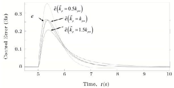
Figure 5. Influence of the proportional gain ( \tilde{k}_p ) on the estimated control error.
