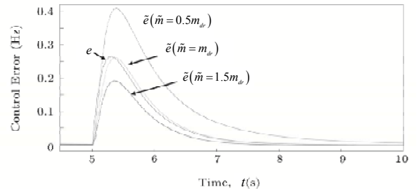
Figure 7. Influence of the droop factor ( \tilde{R} ) on the estimated control error.
