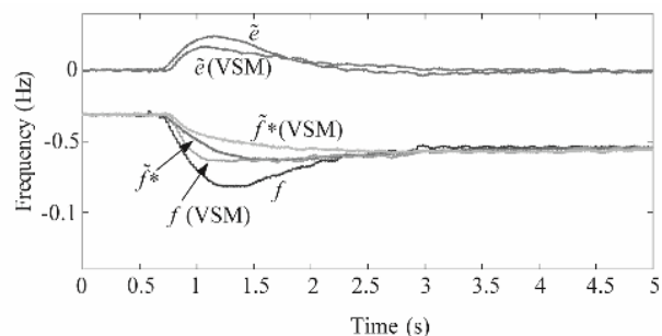
Figure 11. Load increase with gen-set operating with 3% frequency droop.
