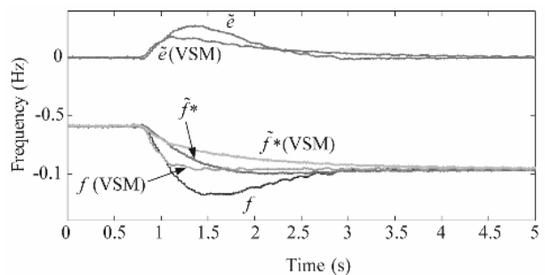
Figure 10. Load increase with gen-set operating with 6% frequency droop.
