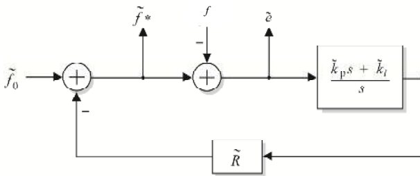
Figure 4. Open-loop estimator.
