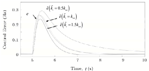
Figure 6. Influence of the integral gain ( \tilde{k}_i ) on the estimated control error.
