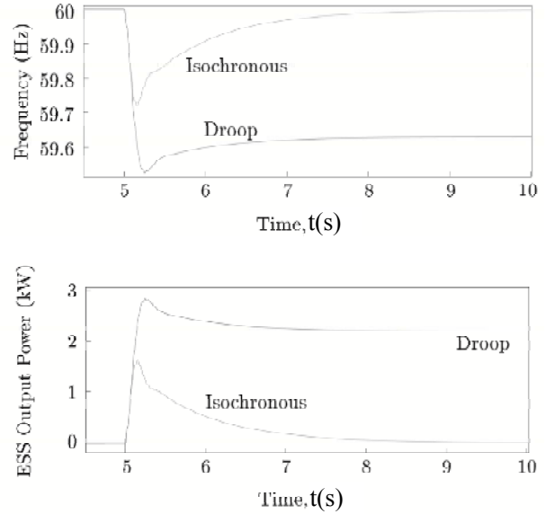
Figure 3. Simulation of the VSM with the gen-set in droop mode. (a) Frequency waveforms; (b) ESS output active power.
