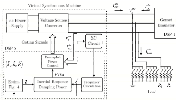
Figure 9. Experimental setup of the VSM with stabilization frequency estimator.
