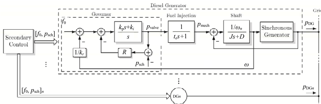
Figure 1. Diesel generator control.
