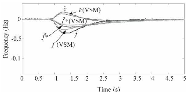
Figure 12. Load increase with gen-set operating in isochronous mode.
