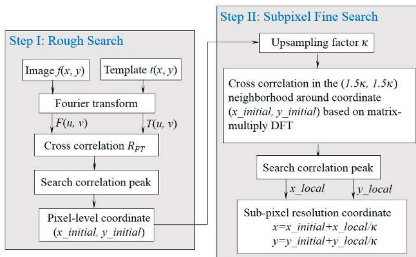
Figure 4. Flowchart of the upsampled cross correlation (UCC) implementation.
