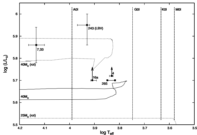
Fig. 5. Location of luminous hypergiants in Wd1 for a distance of 5 kpc compared to z = 0.020 (i.e. solar abundance) evolutionary tracks with and without rotation (Meynet & Maeder 2003). Lower limits for the luminosities of the YHG W4, W16a and W265 are plotted. W4 is offset vertically by 0.02 dex and error bars are omitted for W265 to highlight the change in spectral type over the pulsational cycle.
