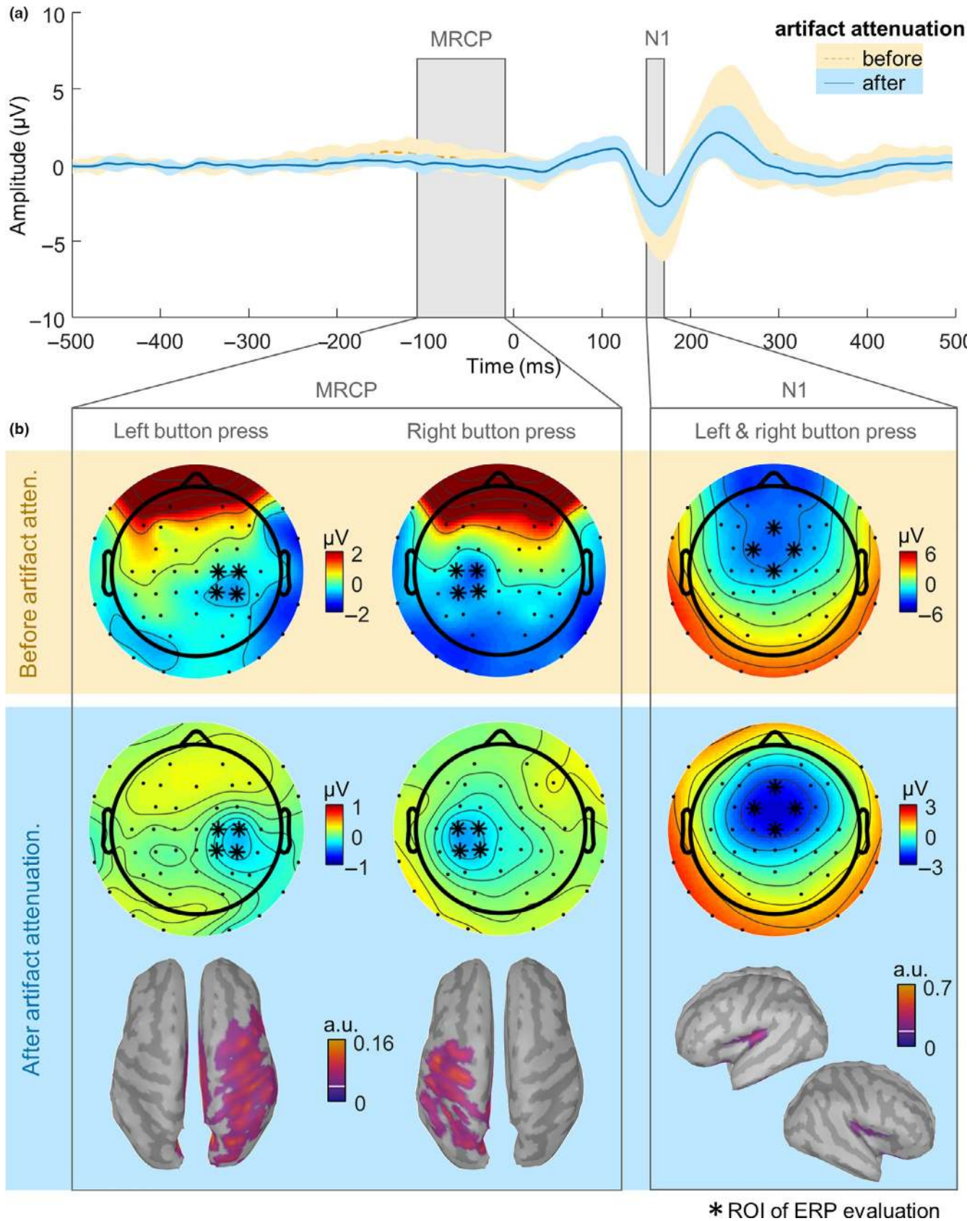
FIGURE 12 (a) Grand mean event-related potential (ERP) of the N1 region of interest (ROI). Time windows of movement-related cortical potential (MRCP) and N1 are marked by grey shaded areas. (b) Topographies of MRCPs and N1 were averaged over intervals indicated in gray in A, before (top row) and after (below) artifact processing. The bottom row illustrates source estimates of the artifact-attenuated group mean response
