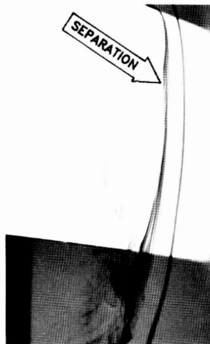
Figure 12. Rectangular wing with small Gurney flap.
