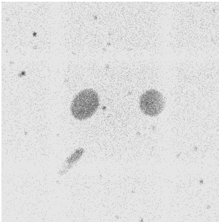
FIG. 11.— Top : 512 \times 512 pixel image (Image A) showing a 1 ks observation by an idealized detector with effective area 1000 \text{ cm}^2 , a spatially invariant Gaussian PSF of width \sigma_{\text{PSF}} = 2.56 pixels, and an exposure map similar to that of the Einstein IPC (§ 4.1). Within this image were placed 42 point sources and four extended sources. The background is assumed to be locally variable, with amplitude \sim 10^{-5} \text{ counts s}^{-1} \text{ pixel}^{-1} . Bottom : same as top, except the observation time is 10 ks (Image B).
