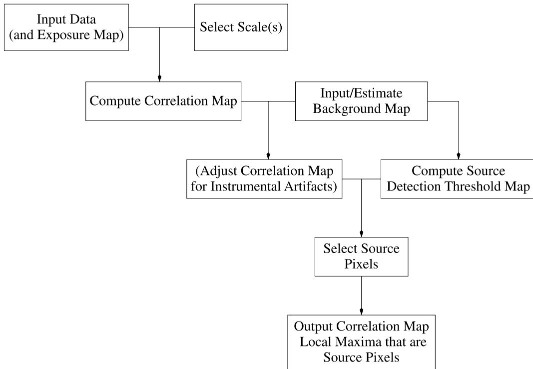
FIG. 2.—Flow chart illustrating the source detection algorithm described in § 3.1, as carried out at selected scales (\sigma_x, \sigma_y) . Parentheses indicate optional input or computations. The local background map may be estimated or provided by the user; a flow chart illustrating how it can be iteratively estimated using the input data (and exposure map) is given in Fig. 3.
