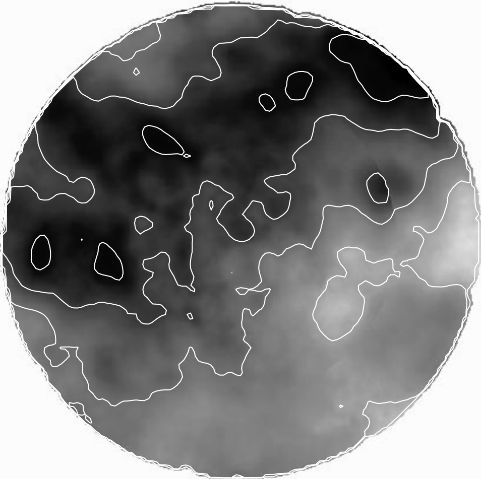
FIG. 17.—Corrected background map generated during the analysis of the ROSAT PSPC image of the Pleiades Cluster (§ 4.2) via the method of § 3.2.1. The contour levels are 0, 0.9, 1.05, 1.2, 1.35, and 1.5 counts, with darker areas having more counts. Since the estimated error in each pixel is \sim 0.01 counts, the perceived structure is real and is indicative of X-ray shadowing (Kashyap et al. 2002, in preparation).
