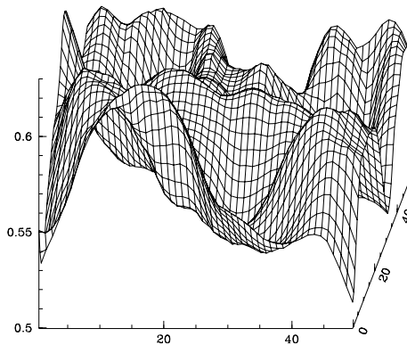
FIG. 4.—Illustration of how source counts may bias a final background estimate (§ 3.1.3), causing “bumps” if the wavelet scale sizes (\sigma_x, \sigma_y) \lesssim r_{\text{PSF}} , the characteristic PSF size at a given pixel. We use a 50 \times 50 subfield of the ROSAT PSPC Pleiades Cluster image in which r_{\text{PSF}} \approx 3 pixels. Top : image and surface plot of the background estimate for \sigma_x = \sigma_y = 1 pixel. Middle : same as top, but for \sigma_x = \sigma_y = 2\sqrt{2} pixels. Bottom : same as top, but for \sigma_x = \sigma_y = 8 pixels.
