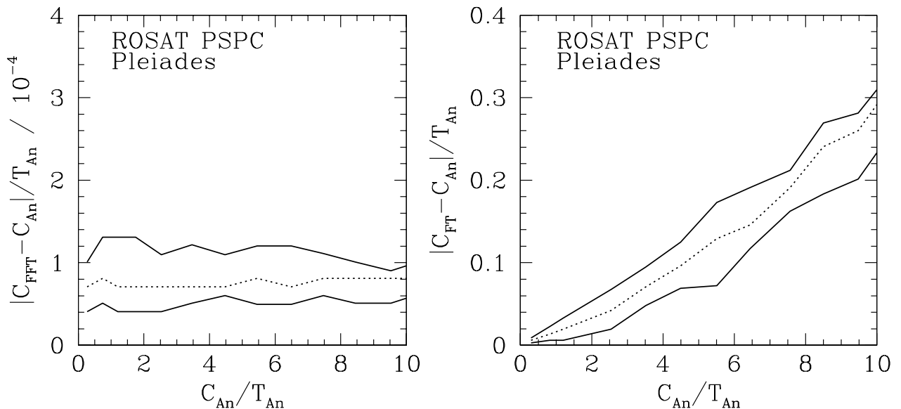
FIG. 22.— Left : discrepancy between the correlation values determined by the analytic method and by using the FFT, for the ROSAT PSPC data of the Pleiades cluster. In this example, \sigma_x = \sigma_y = 2 pixels. Right : same as left, but comparing the analytic method with the use of the analytic Fourier transform for the MH function.
