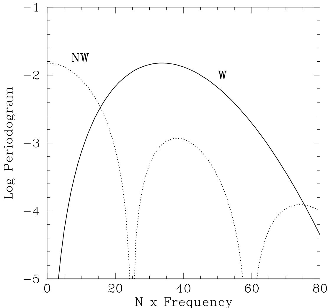
FIG. 6.—Sample power spectra of the Mexican Hat wavelet function ( W ) and of the negative annulus of the Mexican Hat wavelet function ( NW ). N is the number of pixels in the (padded) image. The NW has much larger response to low-frequency components, but this signal would be suppressed upon correlation with W (see § 3.1.4).
