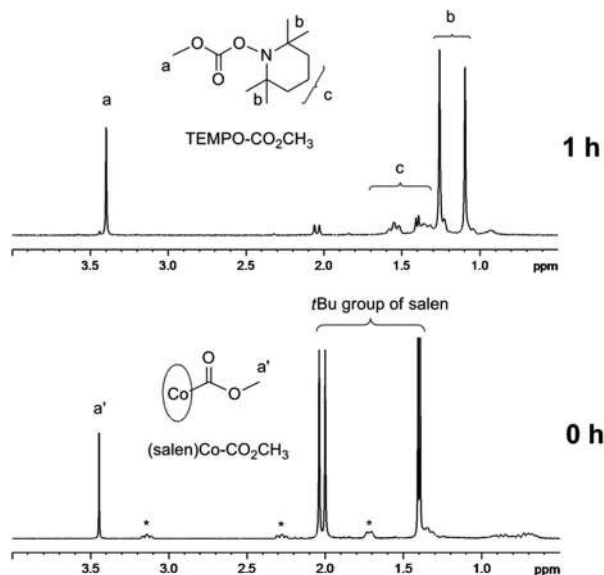
Fig. 2 ^1\text{H} NMR spectra (in the range of 0.5–4.0 ppm) of (salen)Co-CO 2 CH 3 I (5.0 mM) and TEMPO (50 mM) in benzene- d 6 under visible light irradiation ( I = 3 \text{ mW cm}^{-2} at 420–780 nm wavelength) at room temperature for 1 h (*salen ligand in I, see ESI, Fig. 2S†).
