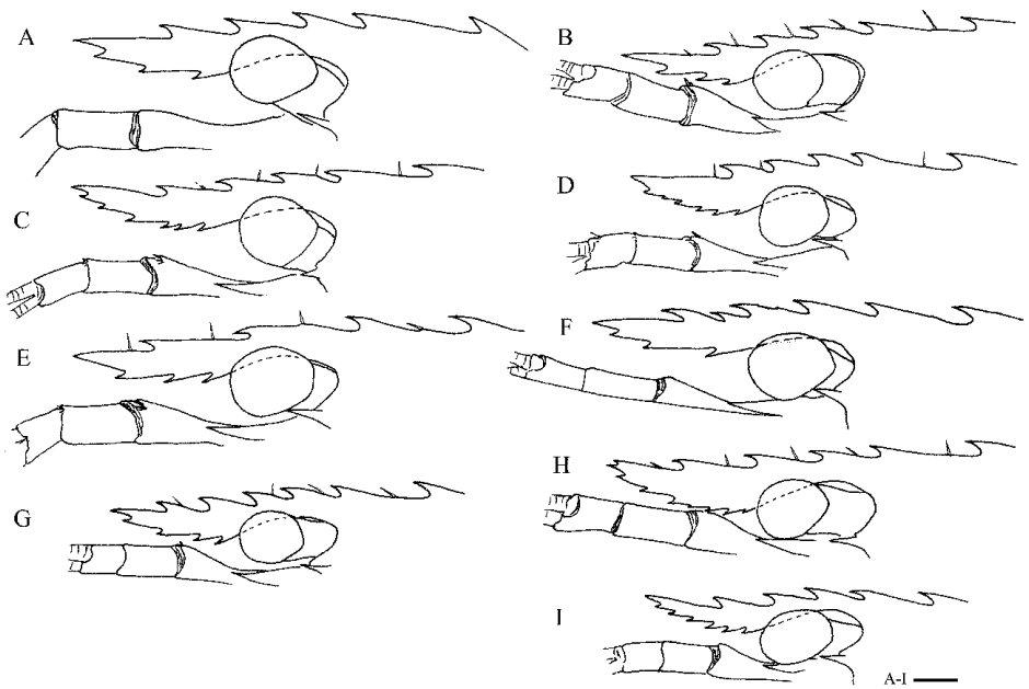
Figure 11. Rostral variation within Lysmata boggeysi new species. (A) USNM 1082807. (B) USNM 1082806. (C-I) USNM 1082805. Scale 1 mm.
