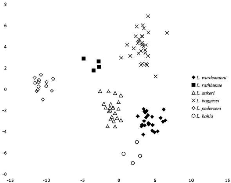
Figure 19. Discriminant Function Analysis (DFA), based on six selected morphological characters of five species in the Lysmata wurdemanni complex and Lysmata rathbunae .
