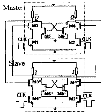
Fig. 2. A Static frequency divider circuit diagram
