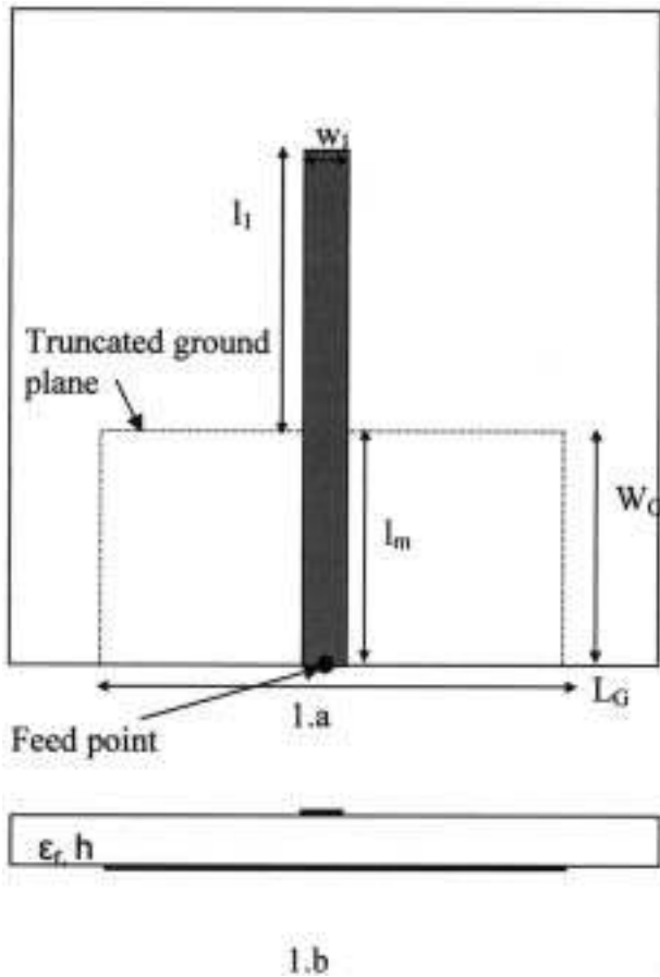
Figure 1 Geometry of the proposed antenna: (a) top view; (b) side view
