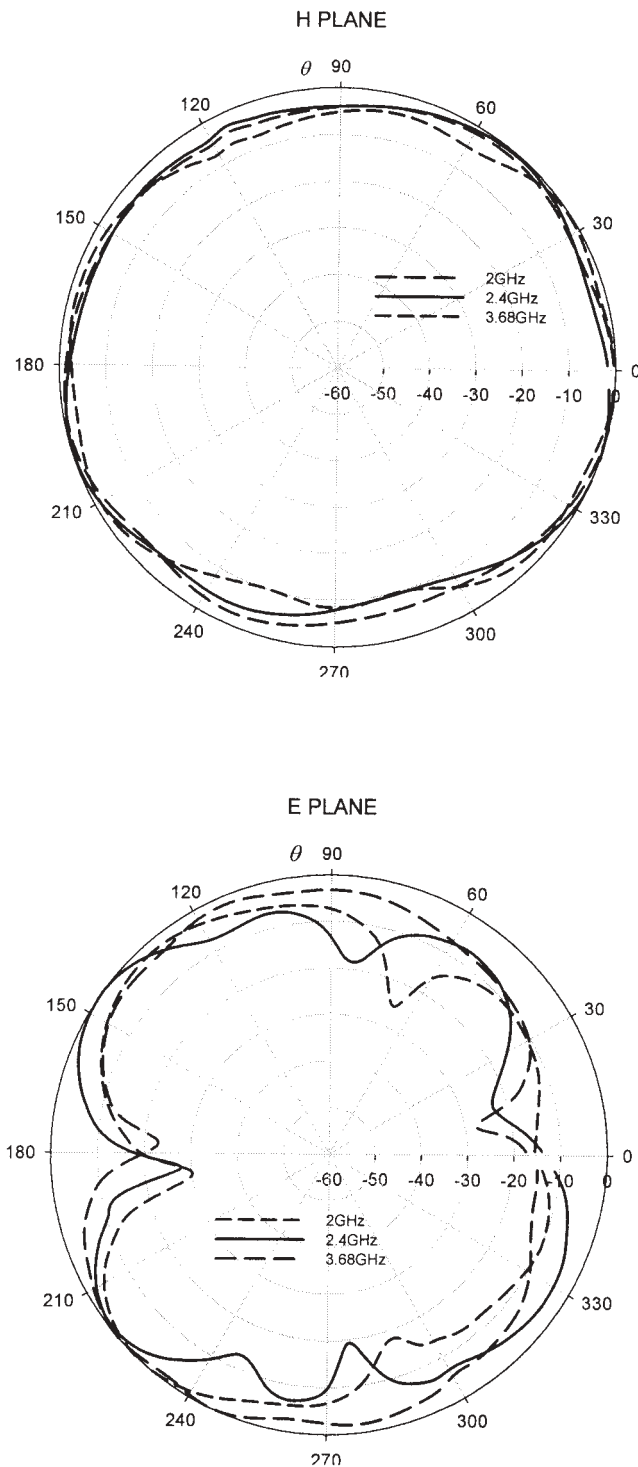
Figure 4 Radiation patterns of the antenna at 2, 2.4, and 3.68 GHz ( L_G = 93 mm, W_G = 43 mm, l_1 = 20 mm, w_1 = 3 mm, \epsilon_r = 4.36 , h = 1.6 mm)
