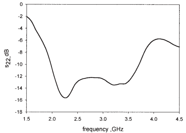
Figure 2 Return-loss characteristics of the antenna at 2.4 GHz ( L_G = 93 mm, W_G = 43 mm, l_1 = 20 mm, w_1 = 3 mm, \epsilon_r = 4.36 , h = 1.6 mm)
