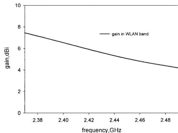
Figure 3 Gain of the antenna at the WLAN band ( L_G = 93 mm, W_G = 43 mm, l_1 = 20 mm, w_1 = 3 mm, \epsilon_r = 4.36 , h = 1.6 mm)
