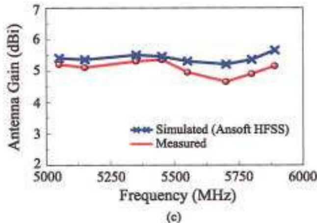
Figure 8 Measured and simulated antenna gain vs. frequency for (a) the first resonant mode, (b) the second resonant mode, and (c) the third resonant mode. [Color figure can be viewed in the online issue, which is available at www.interscience.wiley.com ]
