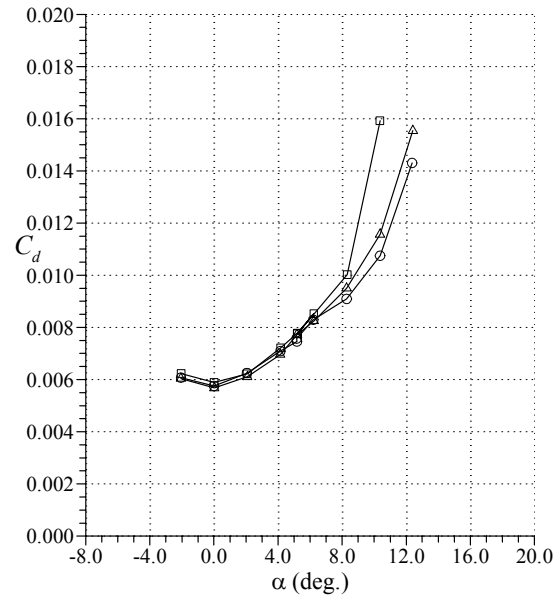
Fig. 7 Effect of Mach number at constant Reynolds number on performance for the clean GLC-305 airfoil.
