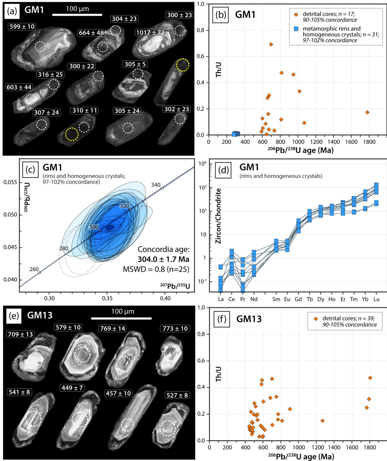
FIGURE 12 (a) Cathodoluminescence images of zircon from garnet-staurolite sample GM1. Dashed white and yellow circles represent the location of the LA-ICP-MS U-Pb (given as ^{206}\text{Pb}/^{238}\text{U} ages) and trace elements analyses, respectively. Zircons in the first and second row display core and rim domains, whereas zircons in the bottom row are internally homogeneous. (b) Th/U ratio versus age plot for sample GM1. (c) Concordia diagram for zircon dates (metamorphic rims and crystals) for sample GM1. Empty dashed ellipses represent data excluded from Concordia age calculation. (d) Trace element compositions of metamorphic zircon rims and homogeneous crystals for garnet-staurolite sample GM1. REE patterns are normalized to chondrite values (McDonough & Sun, 1995). (e) Cathodoluminescence images of zircon from garnet micaschist sample GM13. Dashed white circles represent the location of the LA-ICP-MS U-Pb analyses (given as ^{206}\text{Pb}/^{238}\text{U} ages). (f) Th/U ratio versus age plot for zircon from garnet micaschist sample GM13 [Colour figure can be viewed at wileyonlinelibrary.com ]
