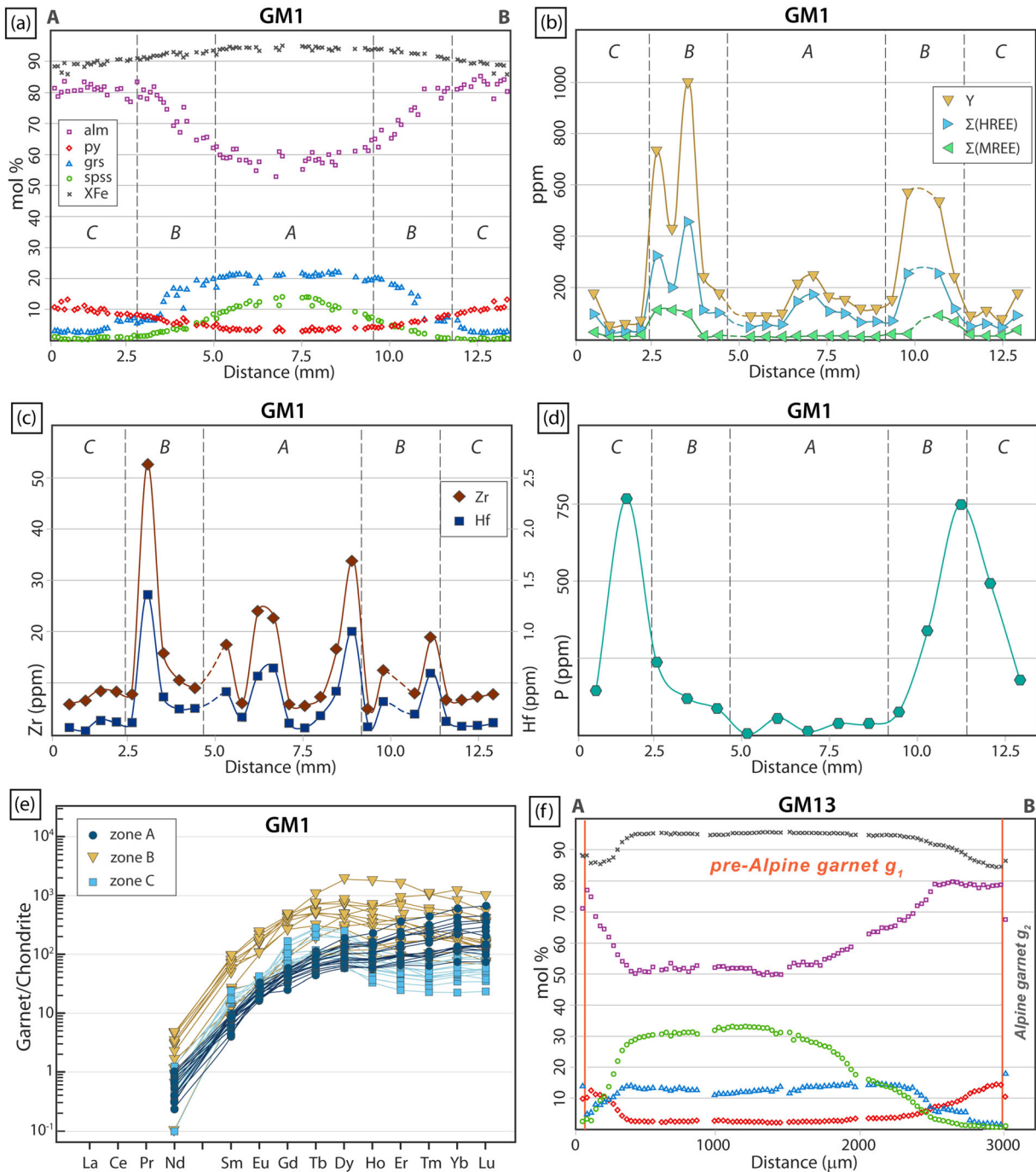
FIGURE 7 Compositional profile of pre-Alpine garnet from garnet-staurolite micaschist (GM1) for major (a) and trace elements (b–d). (b) Compositional profile of Y and sum of HREE and MREE. (c) Compositional profile of Zr and Hf. (d) Compositional profile of P. (e) Chondrite-normalized REE pattern (McDonough & Sun, 1995) for pre-Alpine garnet in sample GM1. (f) Compositional profile of polycyclic garnet from garnet micaschist (GM13) (colour coding as in (a)). Vertical orange lines mark the boundaries between the first and second garnet generations. The position of the profiles (a) and (f) is indicated in Figure 6d and Figure 8e, respectively (lines A–B) [Colour figure can be viewed at wileyonlinelibrary.com ]
