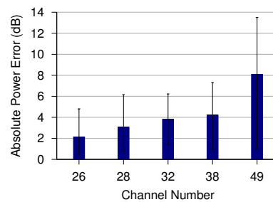
Figure 7: Median error in measuring the power of TV channels by Snoopy. Error bars show 10th and 90th quartile error.
