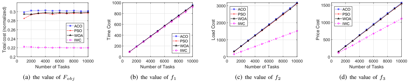
Fig. 6. The best performance achieved of each approach in the large-scale test.
