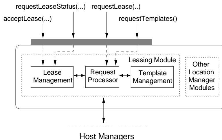
FIG. 3.2. Leasing components within the domain coordinator.
