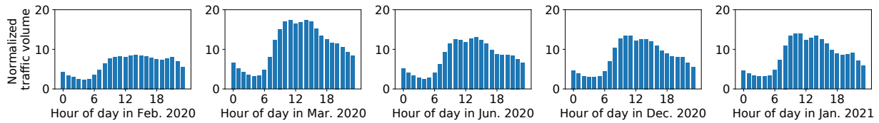
Figure 6: VPN traffic evolution during the COVID-19 pandemic.
