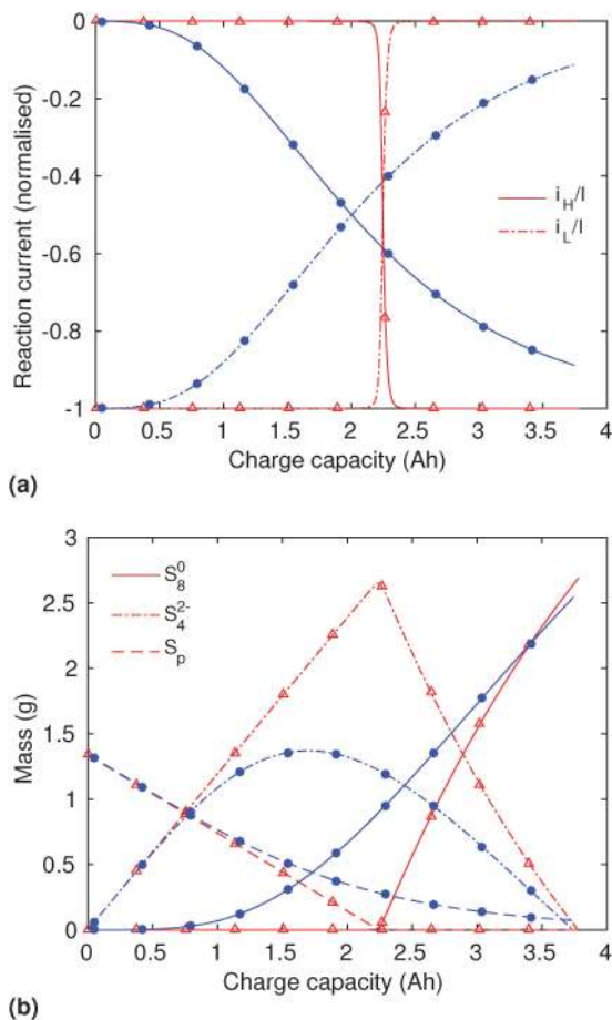
Fig. 4 (a) Simulated reaction currents and (b) species evolution during a 1.7 A (C/2) constant current charge with high saturation concentration S_e^{2-} = 0.005 g, k_p = 100 1/s (red \Delta ) and low saturation concentration S_e^{2-} = 0.0001 g, k_p = 100 1/s (blue \bullet ). The corresponding voltage is illustrated in Fig. 3(b) with the same symbols. The slower dissolution acts as a bottleneck during charge, triggering an earlier onset of the high plateau reaction and eliminating the boundary between the plateaus. Symbols distinguish between data sets rather than denote computed values.
