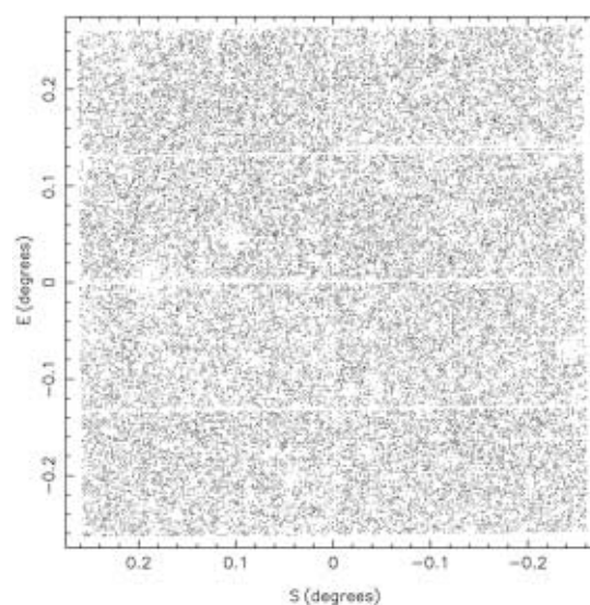
Figure 2 The spatial distribution of stars in the range 22 < r < 24 and 0.5 < g - r < 2.0 for the WFI image of the HVC region. Visible artifacts include the small gaps between the 8 CCDs making up the mosaic imager, regions affected by bad columns, and regions effectively masked out by the light pollution from bright foreground stars in the field. The overall distribution of stars is extremely uniform, with no evidence for any underlying resolved dwarf galaxy population.
