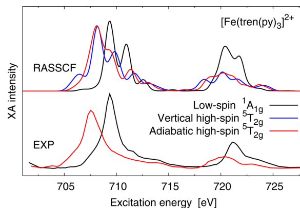
Figure 4. The calculated X-ray absorption spectra of [Fe(tren(py)_3)]^{2+} is compared to the experimental XA spectra 31 of [Fe(tren(py)_3)]^{2+} (singlet ^1A_{1g} ) and a high-spin analogue (quintet ^5T_{2g} ). The RASSCF calculations include core excitations arising from all [(2p)^5, (3d)^7] permutations. A uniform 0.9 eV Gaussian broadening is employed for comparison to experiment.
