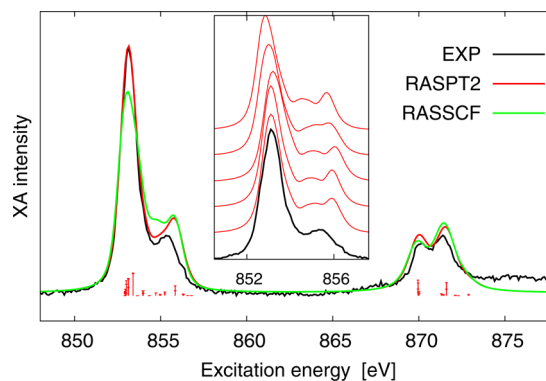
Figure 1. Comparison between the experimental XA spectrum of 1 M \text{NiCl}_2(\text{aq}) solution and XA spectra calculated for \text{Ni}^{2+}(\text{H}_2\text{O})_6 , with the RASSCF and RASPT2 methods. The calculations include core excitations arising from all [(2p)^5, (3d)^9] permutations and the discrete RASPT2 transitions are shown. In the inset, spectra from a configurational sampling are presented.
