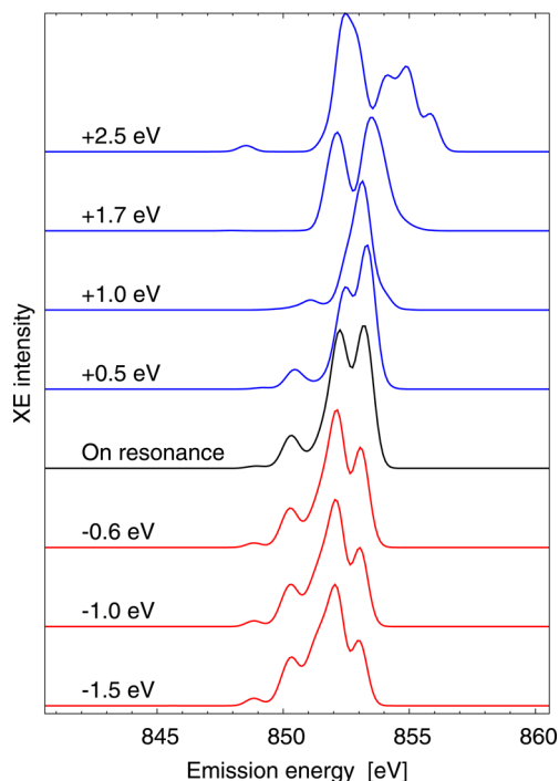
Figure 3. Resonant X-ray emission spectra of Ni^{2+}(H_2O)_6 readily extracted from the RIXS map in panel a in Figure 2, for X-ray excitations energies detuned around the main L_3 edge.
