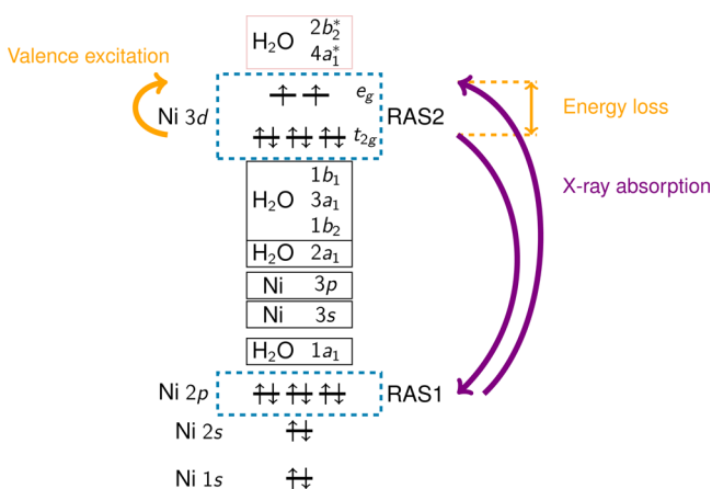
Scheme 1. Molecular orbital diagram of \text{Ni}^{2+}(\text{H}_2\text{O})_6^a
