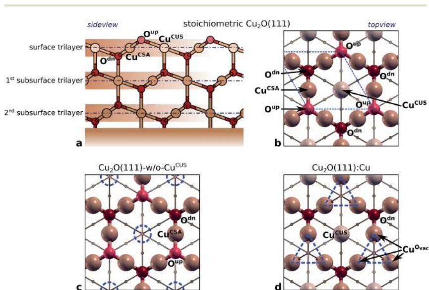
Fig. 7 Structures of various considered \text{Cu}_2\text{O} surfaces (copper and oxygen atoms are colored brownish and reddish, respectively). For clarity of presentation non-relaxed (non-reconstructed) structures are plotted and surface trilayers are emphasized in the top-view plots. (a and b) Side- and top-view of stoichiometric \text{Cu}_2\text{O}(111) ; note the stacking of O–Cu–O trilayers shown in the side view. There are six atoms in the surface trilayer per (1 \times 1) -unit cell [indicated by blue dashed parallelogram in (b)]: 3 \times \text{Cu}^{\text{CSA}} , 1 \times \text{Cu}^{\text{CUS}} , 1 \times \text{O}^{\text{up}} , and 1 \times \text{O}^{\text{dn}} (note that \text{O}^{\text{dn}} is CSA and \text{O}^{\text{up}} is CUS). (c) Non-stoichiometric \text{Cu}_2\text{O}(111) without \text{Cu}^{\text{CUS}} atoms (labeled as \text{Cu}_2\text{O}(111)\text{-w/o-Cu}^{\text{CUS}} ); \text{Cu}^{\text{CUS}} vacancies are indicated by blue dashed circles. (d) Cu terminated \text{Cu}_2\text{O}(111) surface (labeled as \text{Cu}_2\text{O}(111) : \text{Cu} ), which can be seen as stoichiometric \text{Cu}_2\text{O}(111) without \text{O}^{\text{up}} atoms; \text{O}^{\text{up}} vacancies are indicated by blue dashed triangles and the surrounding Cu atoms are labeled as \text{Cu}^{\text{Ovac}} (note that \text{Cu}^{\text{Ovac}} is CUS).
