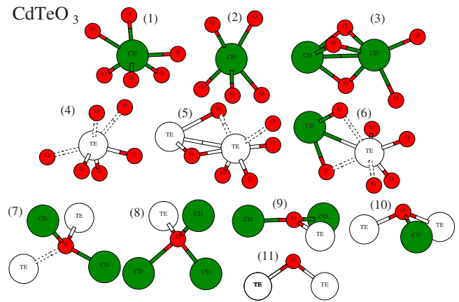
FIG. 14. (Color online) Typical atomic environments in CdTeO 3 . Filled big spheres, empty spheres, and small spheres correspond to Cd, Te, and O atoms, respectively.
