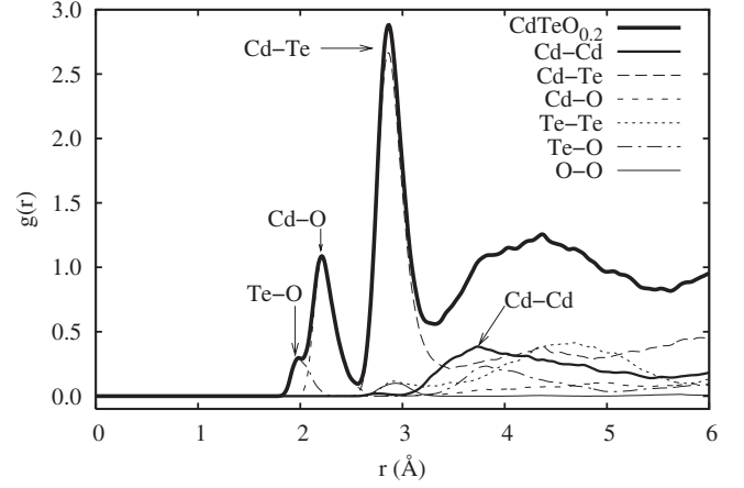
FIG. 1. Total and partial pair distribution functions of \alpha -CdTeO 0.2 .
