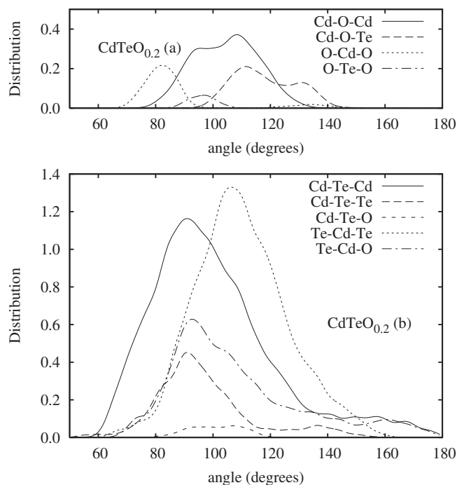
FIG. 4. Angle distribution functions for \alpha -CdTeO 0.2 . In part (a) are the angles involving only Te-O and Cd-O bonds. In part (b) are the angles involving Cd-Te and Te-Te bonds.
