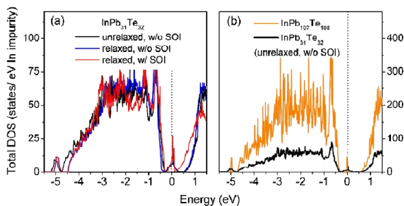
FIG. 2 (color online). Total DOS of (a) \text{InPb}_{31}\text{Te}_{32} with SOI (with ionic relaxation) and without SOI (with and without ionic relaxation), and (b) \text{InPb}_{31}\text{Te}_{32} and \text{InPb}_{107}\text{Te}_{108} (without ionic relaxation, without SOI). Results obtained in PAW calculations. The Fermi level is at 0 eV.
