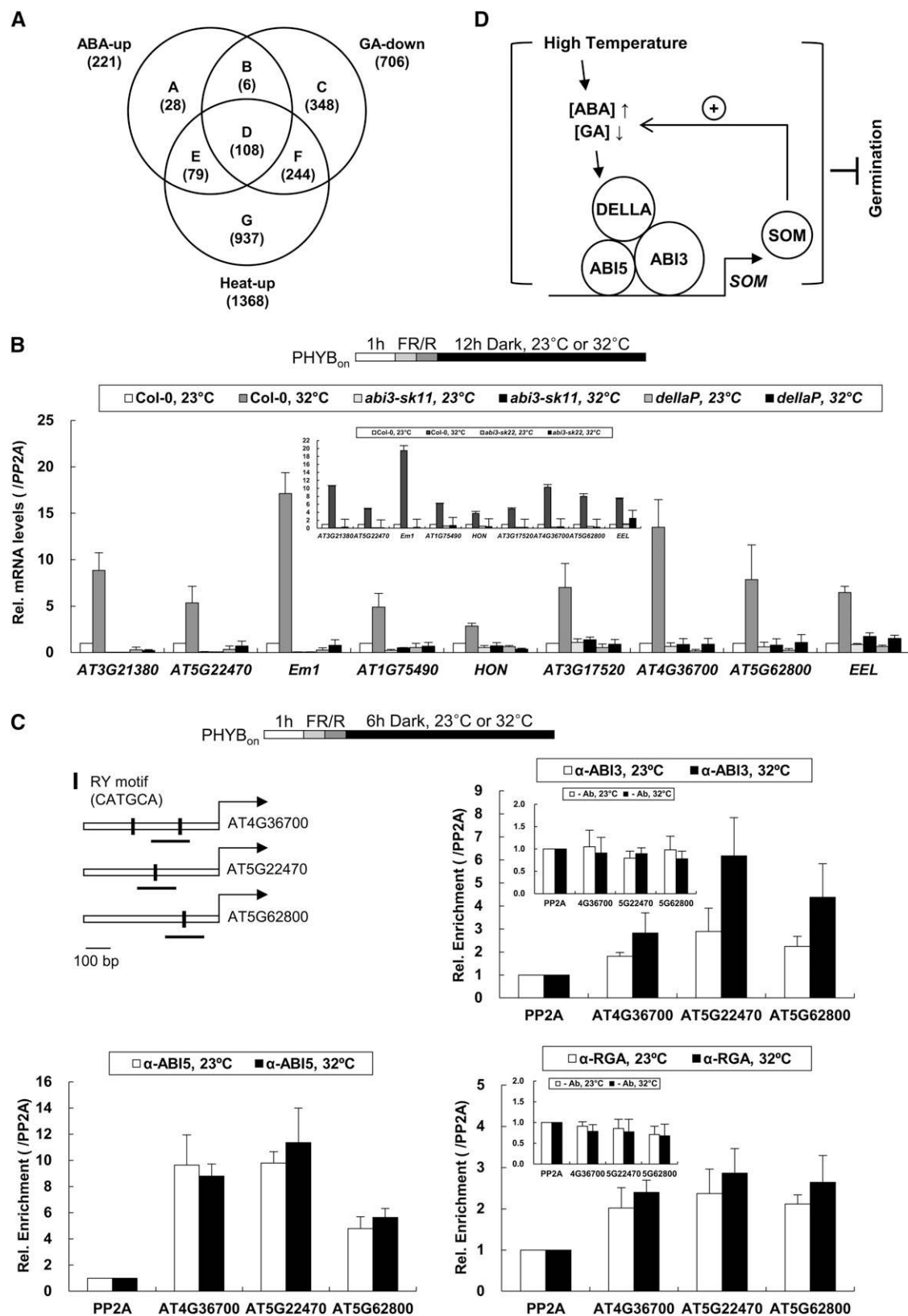
Figure 5. ABI3, ABI5, and DELLAs Mediate ABA and GA Signaling to Activate the Expression of a Subset of High-Temperature-Inducible Genes. (A) A Venn diagram showing numbers of ABA upregulated genes ([ABA-up], \log_2 FC > 0.85, P value < 0.05), GA downregulated genes ([GA-down], \log_2 FC < -0.85, P value < 0.05), and high-temperature-inducible genes ([heat-up], \log_2 FC > 0.85, P value < 0.05), as determined from previously published microarray data (Goda et al., 2008; Chiu et al., 2012). Subsets are indicated by uppercase letters (A to G), and the numbers of genes are given in parentheses.
