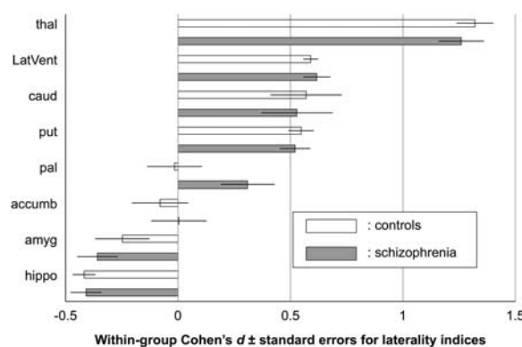
Figure 3. Within-group meta-analytic overall effect sizes (Cohen's d ) \pm standard errors for laterality indices (LIs) of subcortical regional volumes in healthy controls (white bars) and in patients with schizophrenia (gray bars). An LI was defined as the ratio [(left – right)/(left+right)]. In each group, mean LIs and their standard errors were entered into the meta-analysis and an overall mean was obtained. The corresponding forest plots are described in Supplementary Figures 4a–h and 5a–h. An overall effect size for LIs was calculated as the ratio of the overall mean LIs to the overall standard deviation. A positive effect size demonstrates a leftward asymmetry. accumb, accumbens; amyg, amygdala; caud, caudate; hippo, hippocampus; LatVent, lateral ventricle; pal, pallidum; put, putamen; thal, thalamus.
