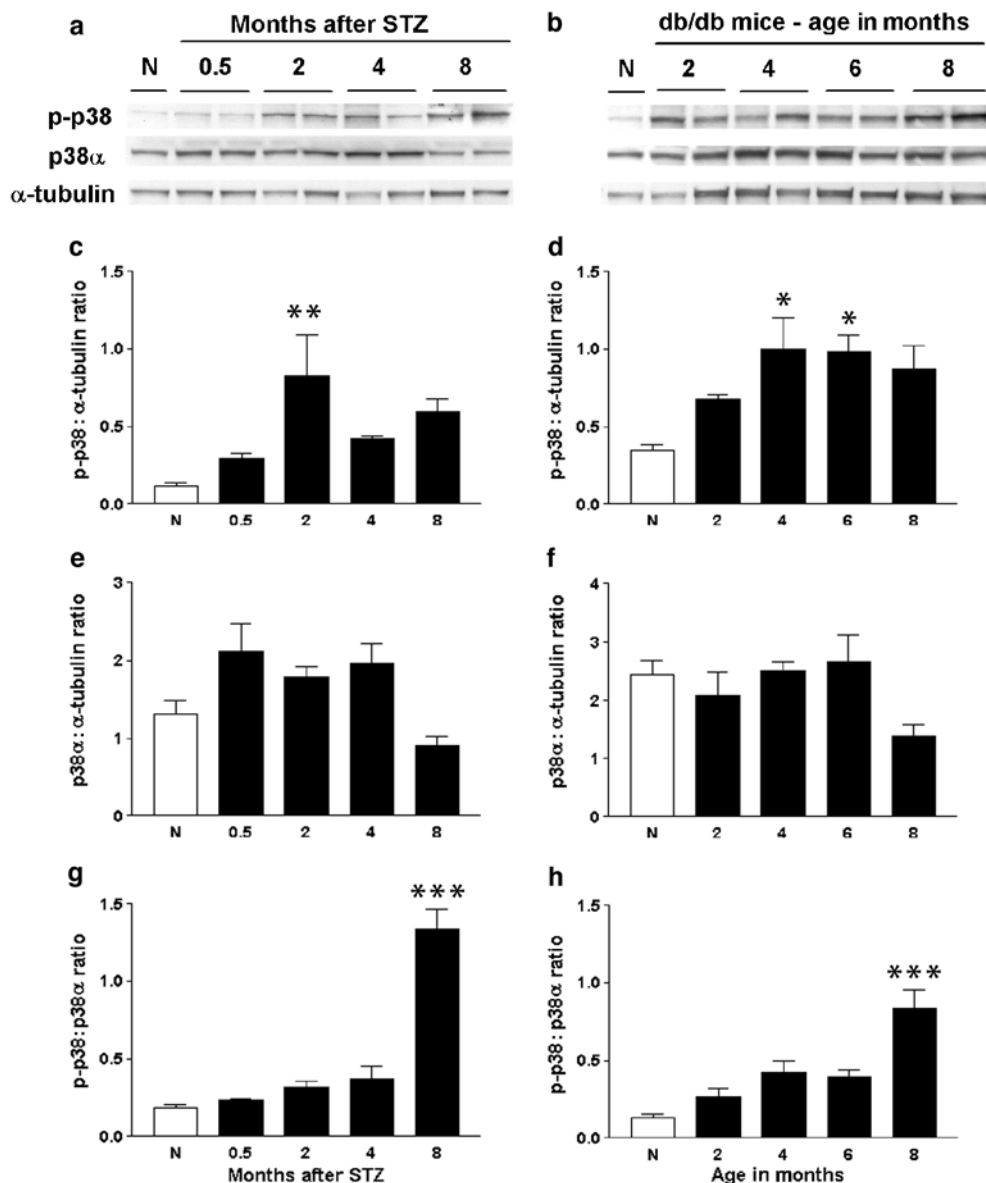
Fig. 3. Increased kidney phosphorylation of p38 MAPK during diabetic nephropathy. Western blots detected greater levels of p-p38 in total kidney lysates from (a) streptozotocin (STZ)-treated diabetic mice and (b) db/db diabetic mice than in lysates from normal mice (N). Kidney levels of \alpha -tubulin were used as a loading reference. Kidney levels of p-p38 increased rapidly during the early stages of diabetic nephropathy in STZ-treated mice (c) and db/db mice (d). In comparison, kidney levels of p38 \alpha remained relatively unchanged throughout in STZ-treated mice (e) and db/db mice (f). Comparison of p-p38 with p38 \alpha levels showed a significant increase in the kidney p-p38 : p38 \alpha ratio in advanced stages of diabetic nephropathy in STZ-treated mice (g) and db/db mice (h). Data are mean \pm SEM, n=4 ; * p<0.05 , ** p<0.01 , *** p<0.001 vs normal by ANOVA
