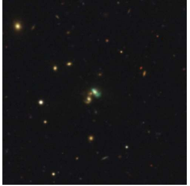
Figure A17. J2240–0927.
