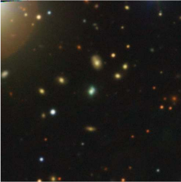
Figure A14. J2050+0550.
