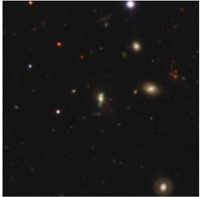
Figure A2. J0024+3258.
