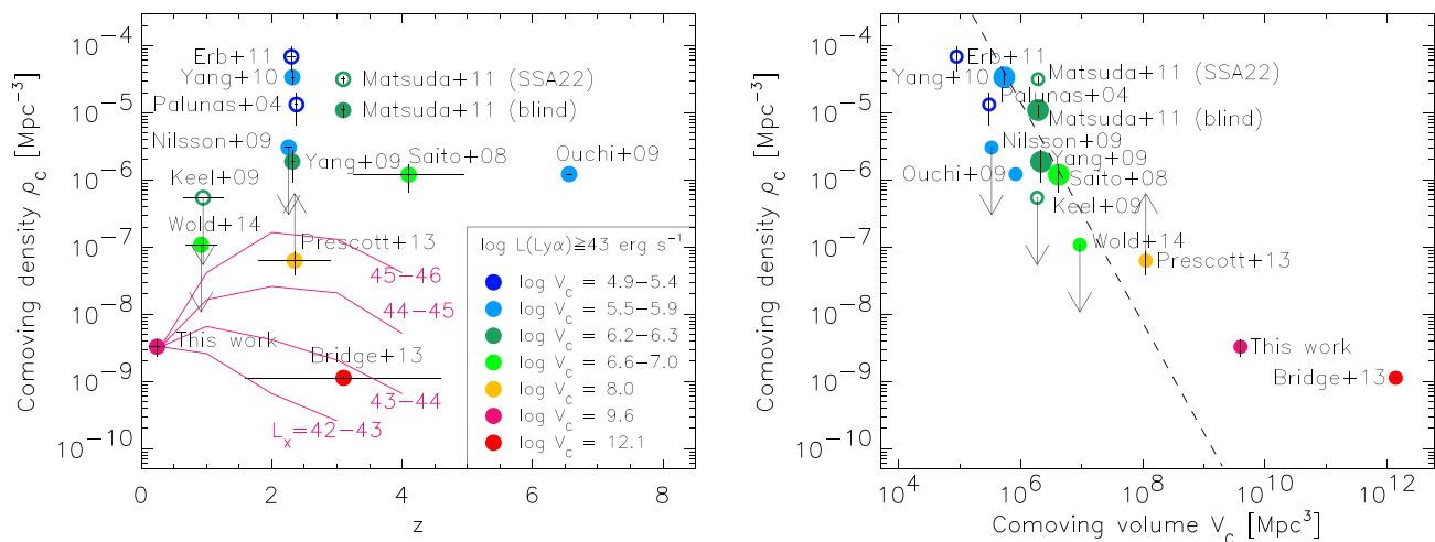
Figure 6. Left: comoving density of LABs ( L_{\text{Ly}\alpha} \geq 10^{43} \text{ erg s}^{-1} , D \geq 20 \text{ kpc} ) as a function of redshift. Filled dots represent blind surveys and open dots cluster areas. Horizontal lines show the redshift range covered; vertical lines are the Poisson errors. Arrows represent upper limits. Symbol colours display the survey comoving volumes (see also the right-hand panel). The pink lines show how GBs evolve for different X-ray luminosities if linked to the AGN density evolution. Right: comoving density as a function of the surveys’ comoving volume. There should be no dependence on volume if the surveys are independent of the environment. The dashed line shows the best fit to the blind surveys at z = 2-4 (larger filled dots). We kept the colour coding for easier comparison with the left-hand panel.
