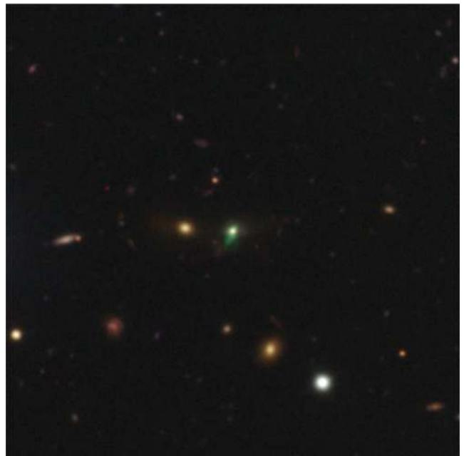
Figure A3. J0111+2253.
