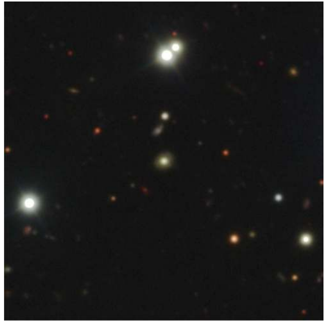
Figure A18. J2308+3303.
