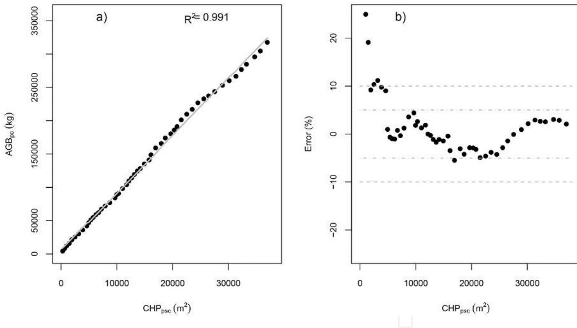
Figure 5. Cumulative values of crown horizontal projection derived from satellite image per plot (CHP p,c ) versus cumulative values of above-ground biomass per plot (AGB p,c ) and equation (in grey, a), and error distribution (b) for model 14.
