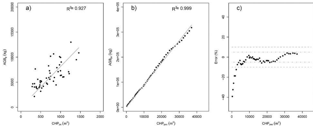
Figure 4. Crown horizontal projection derived from satellite image per plot (CHP ps ) versus above-ground biomass per plot (AGB p ) and equation (in grey) for model 9 (a) and their cumulative values, CHP p,c vs AGB p,c , and equation (in grey) (b) and error (c) for model 12.
