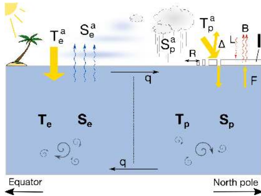
Figure 2. Schematic of the coupled sea ice–ocean model including model parameters and variables (bold). A description of the parameters is given in Table 1. The well-mixed polar and equatorial ocean boxes are coupled by a surface flow q , along with an identical return flow at the bottom. The ocean component is reduced to the two variables T \propto T_e - T_p and S \propto S_e - S_p . In the polar ocean box, the sea ice cover I insulates the ocean from the cold atmospheric temperature T_p^a .
