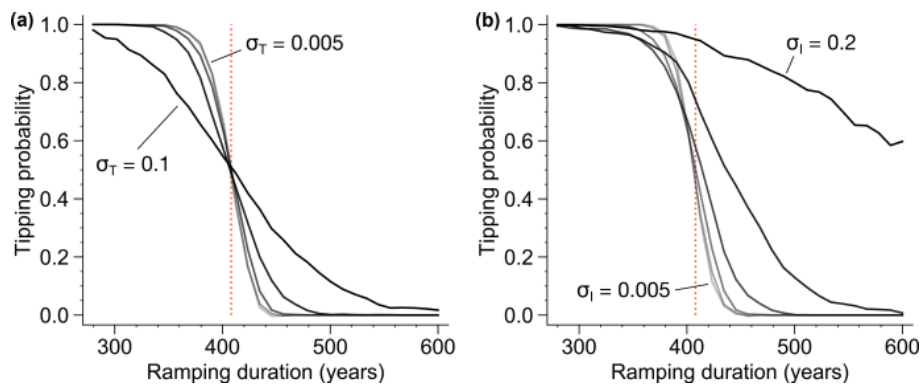
Figure 11. Probability of a cascading transition in the coupled sea ice–ocean model when changing the control parameter R linearly from R = 0 to R = -0.3 within different ramping times. (a) Fixed noise level \sigma_I = 0.02 in the sea ice component and varying noise levels \sigma_T = \sigma_S = \sigma = 0.005 (lightest gray), \sigma = 0.01 , \sigma = 0.02 , \sigma = 0.04 and \sigma = 0.1 (darkest gray) in the ocean component. (b) Fixed noise level \sigma_T = \sigma_S = 0.02 in the ocean component and varying noise levels \sigma_I = 0.005 (lightest gray), \sigma_I = 0.01 , \sigma_I = 0.02 , \sigma_I = 0.04 , \sigma_I = 0.08 and \sigma_I = 0.2 (darkest gray) in the sea ice component.
