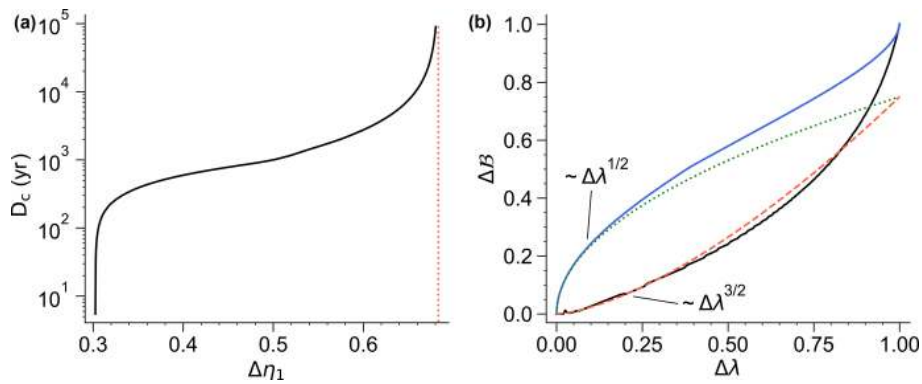
Figure 7. (a) Critical ramping duration below which there is a rate-induced tipping in the Stommel model when shifting the parameter from \eta_1 = 2.65 to \eta_1 = 2.65 + \Delta\eta_1 . The off attractor loses stability in the bifurcation at \eta_1^{\text{off}} = 3.333 , as indicated by the dashed red line. (b) Normalized shortest distance to the basin boundary \Delta\mathcal{B} as a function of the normalized distance to the bifurcation \Delta\lambda = (\eta_1^{\text{off}} - \eta_1) \cdot (\eta_1^{\text{off}} - \eta_1^{\text{on}})^{-1} . \eta_1^{\text{on}} is the parameter value at the other saddle node bifurcation of the on state. The solid black curve shows the results of the Stommel model, and a proposed super-linear scaling is shown by the dashed curve. Also shown are results for the smooth bifurcation in the sea ice component (solid blue) and the corresponding square-root scaling (dotted).
