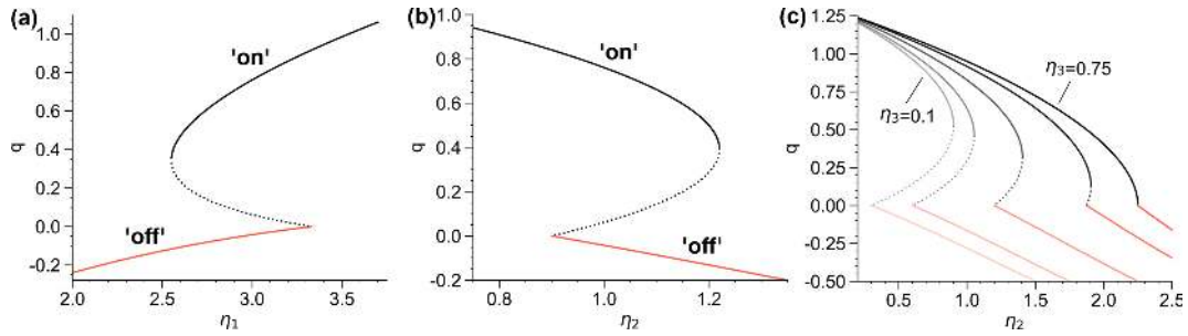
Figure 1. (a) Bifurcation diagram of the Stommel box model with \eta_1 as control parameter, \eta_2 = 1.0 and \eta_3 = 0.3 . Solid lines indicate branches of stable fixed points, whereas dotted lines indicate unstable fixed (or saddle) points. (b) Bifurcation diagram with \eta_2 as control parameter, \eta_1 = 3.0 and \eta_3 = 0.3 . (c) Dependence of bi-stability interval on \eta_3 ( \eta_1 = 3.0 ). The individual bifurcation diagrams with \eta_2 as control parameter are shown with decreasing bistability interval as \eta_3 is increased from 0.1 up to 0.75.
