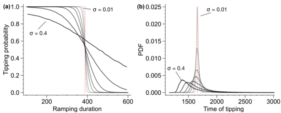
Figure 8. (a) Probability of a rate-induced tipping in the Stommel model from the off to the on state as a function of the linear parameter ramping duration from \eta_1 = 2.65 to \eta_1 = 3.00 . Different noise levels \sigma_T = \sigma_S = \sigma are considered: \sigma = 0.01 (lightest gray curve), \sigma = 0.02 , \sigma = 0.04 , \sigma = 0.06 , \sigma = 0.1 , \sigma = 0.2 , and \sigma = 0.4 (darkest gray curve). The dashed red line is the critical ramping duration in the deterministic system. (b) Probability distributions of the time of tipping, defined by the first crossing of q > 0.1 , for different noise levels. The ramping is started in year 1000 and the duration is fixed at 300 years. The dashed red line is the time of tipping in the deterministic system.
