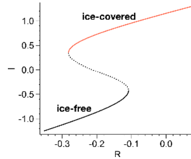
Figure 3. Bifurcation diagram of the sea ice component for parameter values as in Table 1. The solid (dotted) lines indicate stable (unstable) fixed points.
