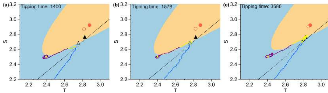
Figure 9. (a–c) Three realizations in phase space of the Stommel model with \sigma_T = \sigma_S = 0.2 , where \eta_1 is ramped from \eta_1 = 2.65 to \eta_1 = 3.00 over 300 years. The filled dot (triangle) marks the off fixed point (saddle) at \eta_1 = 3.0 . The colored areas are the quasi-stationary basins of attraction at the time when their boundary is first crossed. The colored basins of attractions are given at the time of first basin crossing of the trajectories, which change color from purple to yellow. The initial conditions T, S = (2.4, 2.5) are indicated by the yellow cross. The locations of the saddle point (triangle) and the on fixed point at this time are shown with open symbols. The threshold q = T - S = 0.1 used to define the time of tipping is shown as a dotted line.
