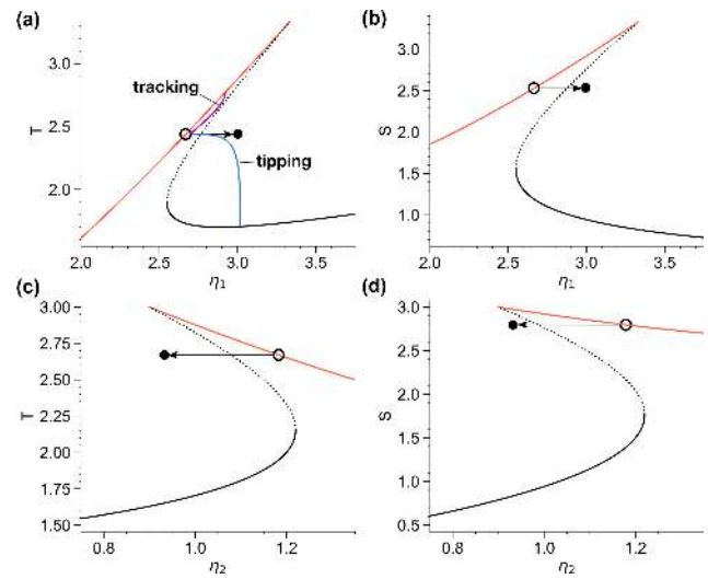
Figure 4. (a, b) Bifurcation diagram of the Stommel model equilibria in terms of the variables (a) T and (b) S as a function of \eta_1 as control parameter with \eta_2 = 1.0 and \eta_3 = 0.3 . (c, d) The same as (a, b) but with \eta_2 as control parameter with \eta_1 = 3.0 and \eta_3 = 0.3 . Solid lines indicate stable fixed points, whereas dotted lines indicate saddle points. The horizontal arrows indicate the movement of the system state as the control parameter is changed instantaneously within the bi-stable regime. In (a) we illustrate how the system state may track the moving equilibrium for a slow parameter shift (purple trajectory) or tip to the undesired equilibrium in a fast parameter change (blue trajectory).
