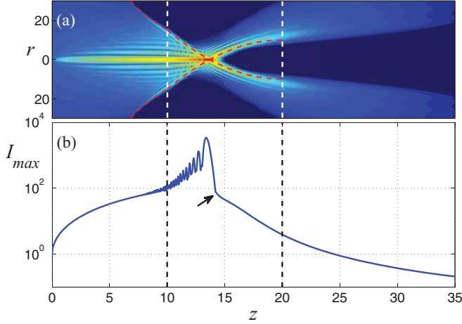
FIG. 4. (Color online) (a) Amplitude evolution of a beam with the same parameters with Fig. 3 but with the complex conjugate input amplitude. The dashed curves indicate the caustics. (b) Maximum intensity versus propagation distance. The arrow indicates the point where the AADF ends. The dashed vertical lines indicate planes z = f and z = 2f .
