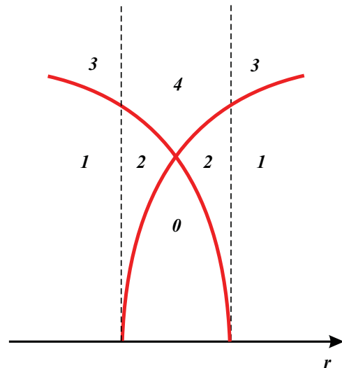
FIG. 8. (Color online) Regions for ray optics computations of the field of an AAF wave. The regions are characterized by the number of rays contributing to the field at any point.
