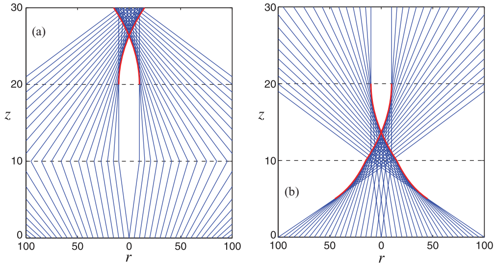
FIG. 2. (Color online) Ray patterns on a vertical plane for a beam with input phase: (a) \alpha r + br^n and (b) -\alpha r - br^n , with parameters n = 3 , a = 1 , b = 1/3000 , and a lens with f = 10 . The red curves (ray envelopes) are the caustics, while the dashed horizontal lines indicate the lens' plane ( z = f ) and the image plane ( z = 2f ).
