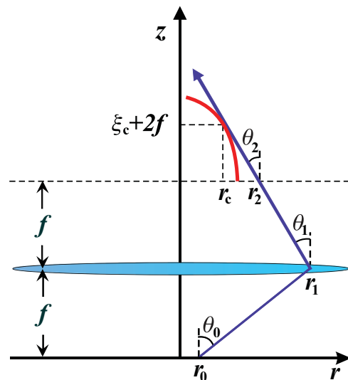
FIG. 1. (Color online) Schematic of a ray traveling through a single-lens FT system. The lens is positioned at z = f . The red (convex) curve indicates the caustic formed beyond z = 2f .
