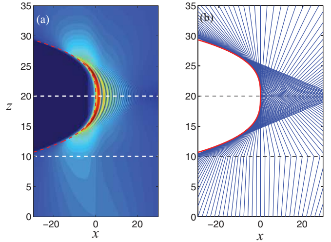
FIG. 6. (Color online) (a) Amplitude evolution of a 1D beam with parameters n = 5/2 , a = 0 , b = 0.00253 , a Gaussian input envelope with e^{-1} width 90 and a lens with f = 10 . The envelope curve is the caustic, while the dashed horizontal lines indicate the lens and image planes. (b) Corresponding ray pattern.
