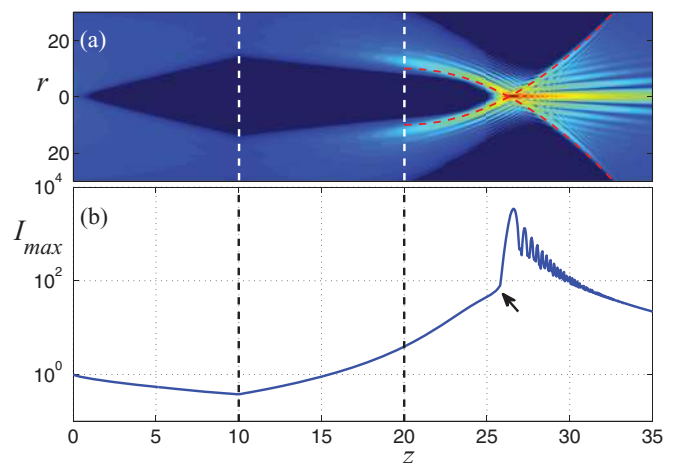
FIG. 3. (Color online) (a) Amplitude evolution of a beam with Gaussian input envelope with e^{-1} radius w = 45 and the phase modulation parameters of Fig. 2(a). The dashed curves are the caustics of Eq. (11). (b) Maximum intensity versus propagation distance. The arrow indicates the point where the AAF starts. The dashed vertical lines indicate planes z = f and z = 2f .
