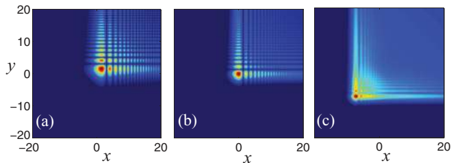
FIG. 7. (Color online) Transverse amplitude at different z planes of an accelerating 2D beam produced by Fourier-transforming the input wavefront u_0(x, y) = A(x)A(y) \exp[i\Phi(x) + i\Phi(y)] , with A(u) = \exp[-(u/45)^2] and \Phi(u) = 0.00253 \text{sgn}(u)|u|^{5/2} . (a) z = 20 , (b) z = 23 , (c) z = 26 . The lens has f = 10 .
