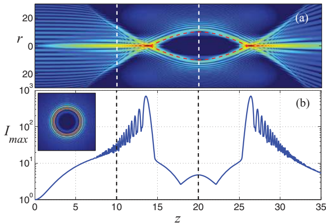
FIG. 5. (Color online) (a) Amplitude evolution of a beam with input amplitude \exp[-(r/45)^2] \cos[\Phi(r)] , where \Phi is given by Eqs. (14) and (15) for \kappa = \pi/12 , a = 1 , f = 10 . The dashed curves indicate the sinusoidal part of the caustic. (b) Maximum intensity versus propagation distance. The dashed vertical lines indicate planes z = f and z = 2f . The inset shows the amplitude distribution on the image plane.
