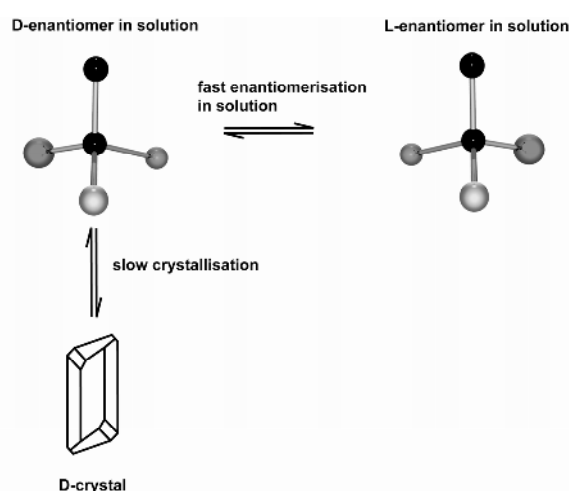
Figure 3-10. An equilibrium between the two enantiomers in solution may give rise to total spontaneous resolution, since equal amounts of D and L -crystals are not necessarily formed. If primary nucleation starts with e.g. a D -nucleus, D -crystals will start to grow and the entire amount of solute may successively be converted to the D -enantiomer and no L -crystals are obtained.
