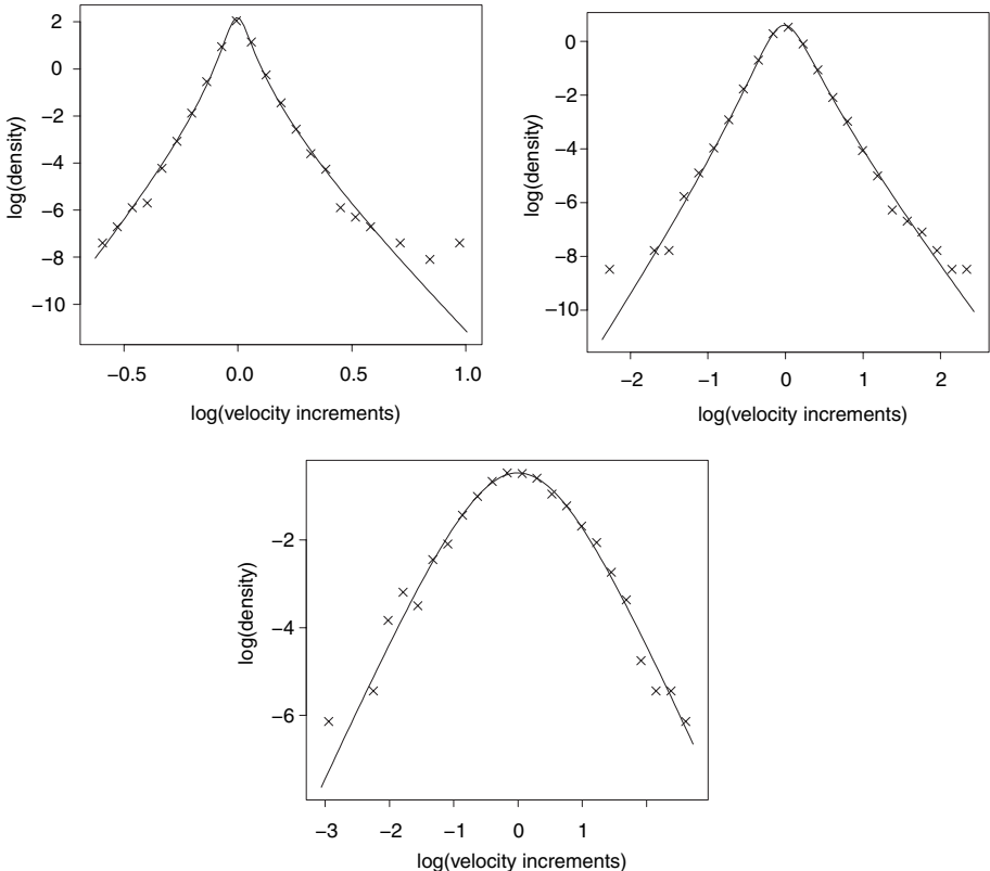
Fig. 1. Log-density (solid line) of NIG distribution fitted to velocity increments at lags 12 (upper left), 500 (upper right) and 9000 (lower centre) and log-histogram (only top end points are given (x)).
