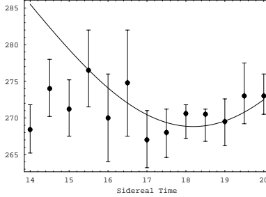
Figure 18: Frequency difference in kHz between the two masers in the 1963 New Bedford experiment after a 90^0 rotation. The 275kHz difference is a systematic repeatable apparatus effect, whereas the superimposed ‘dip’ at 17 – 18:00 hr sidereal time of approximately 3kHz is a real time dependent frequency difference. The full curve shows the theoretical prediction for the time of the ‘dip’ for this experiment using the Miller direction for \hat{\mathbf{v}} ( \alpha = 5.2^{hr} , \delta = -67^0 ) with |\mathbf{v}| = 433\text{km/s} and including the earth’s orbital velocity and sun gravitational in-flow velocity effects for January 20, 1963. The absolute scale of this theoretical prediction was not possible to compute as the refractive index of the He-Ne gas mixture was unknown.
