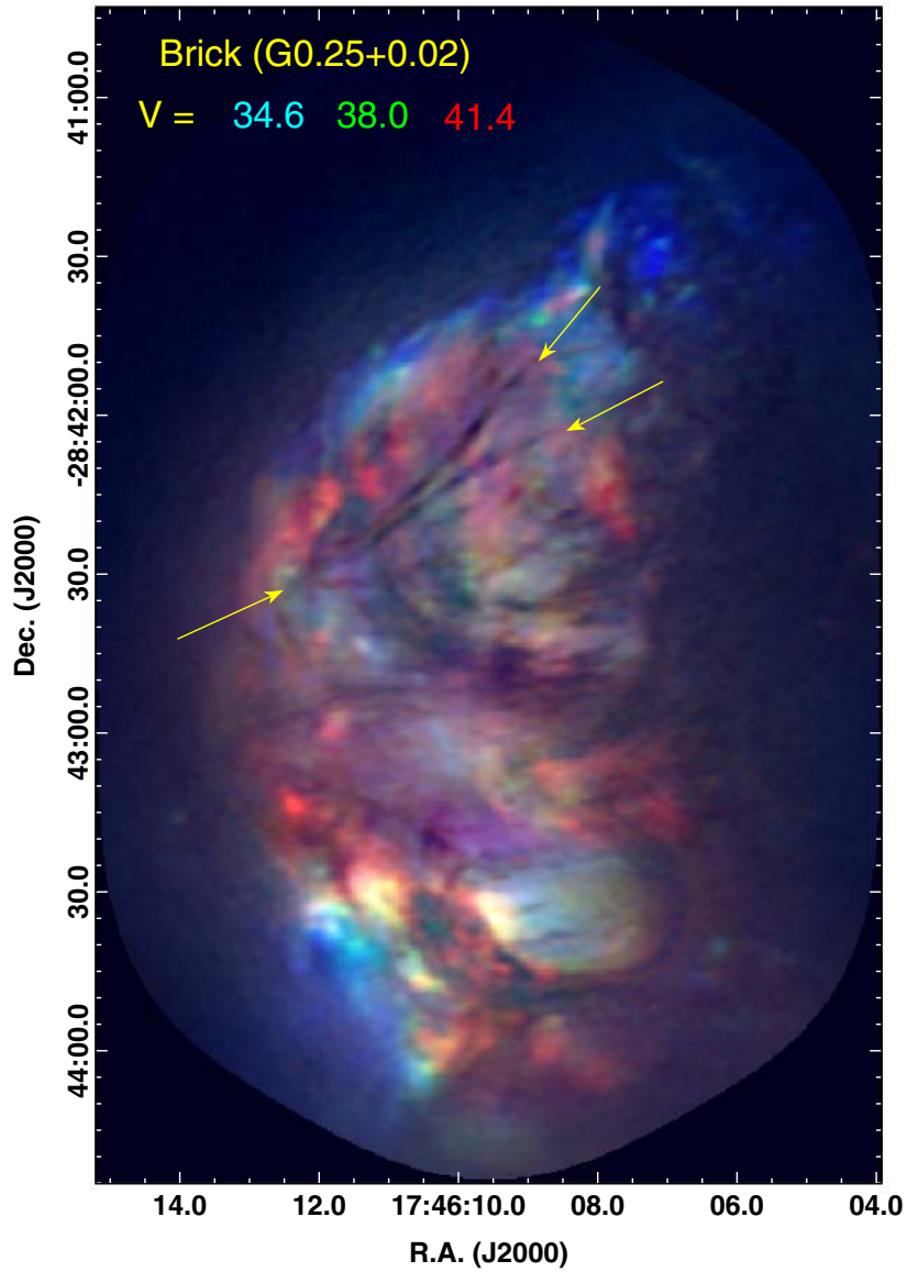
Figure 6. This figure shows HCO + channels centered at V_{\text{LSR}} = 34.6 (blue), 38.0 (green), and 41.4 (red) km s -1 . (A color version of this figure is available in the online journal.)
