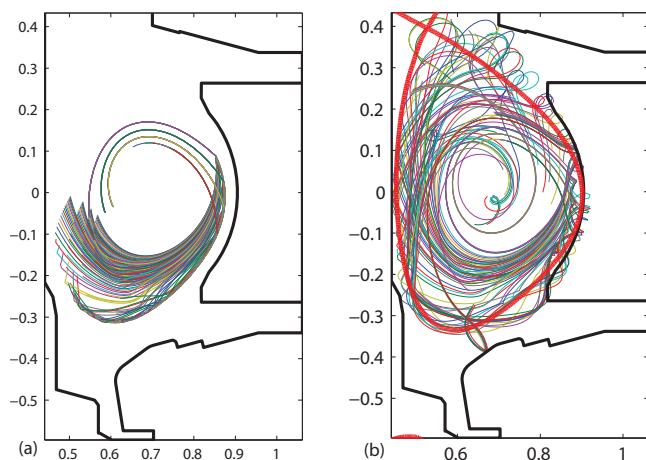
FIG. 13. (Color online) (a) GENRAY simulation showing rays trapped near the edge of the plasma. Each ray corresponds to a specific launch location and launched value of n_{\parallel} . The highest n_{\parallel} rays penetrate to near the core of the plasma, while the lower n_{\parallel} rays stay close to the edge. Rays propagating in the current drive direction move downward from the low field side (LFS) launch point, while rays propagating in the countercurrent drive direction move upward from the LFS launch point. The cutoff layer in this simulation is located at the separatrix and the vacuum vessel walls are superimposed for reference. The rays are truncated for clarity after a fixed distance. (b) Ray trajectories including a 2D SOL model and reflections from the vacuum vessel. The separatrix location is indicated by a bold line. \sigma_T(\theta) is estimated on the basis of flux expansion.
