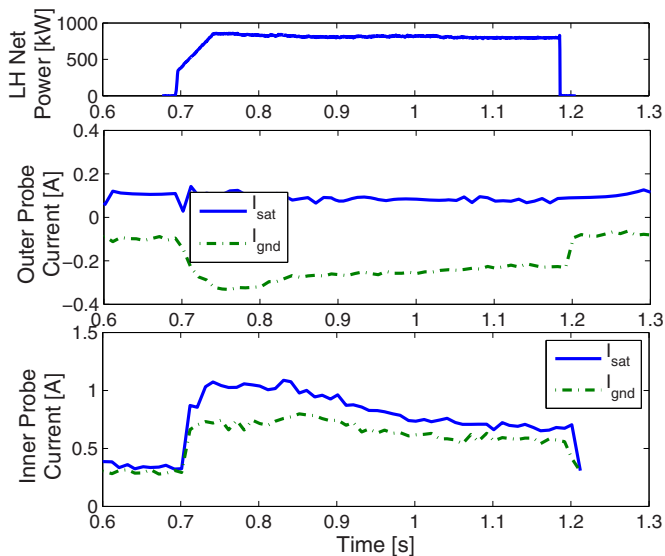
FIG. 11. (Color online) Comparison of I_{\text{gnd}} and I_{\text{sat}} on divertor probes in LSN configuration. I_{\text{gnd}} on the inner divertor is near the limit set by I_{\text{sat}} , while on the outer divertor |I_{\text{gnd}}| exceeds |I_{\text{sat}}| . Shot number=1080402031.
